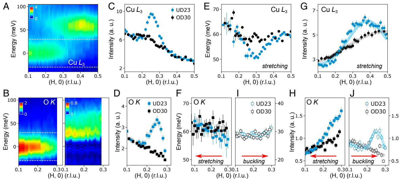
Fig. 3. CDW and phonons studies in overdoped OD30. ( A and B ) \text{Cu } L_{3-} and \text{O } K RIXS intensity map as a function of energy and q_{\parallel} along the (H, 0) direction, respectively. The map on the right-hand side of B is the residual excitations after subtraction of the fitted elastic peaks. ( C and D ) Integrated intensities of the quasielastic peaks at the \text{Cu } L_{3-} (black dots) and \text{O } K (black squares) within the energy window ( \pm 30 meV) defined by the two white dashed lines in A and B . Integrated elastic peaks intensities in UD23 from the same energy range are shown in blue for comparison. ( E ) Dispersion of the bond-stretching phonon excitations at the \text{Cu } L_{3-} in OD30 (black dots) extracted from the fitting. ( F and I ) Dispersion of the bond-stretching phonon (black filled squares) and bond-buckling phonon (black open squares) excitations at the \text{O } K edge. For E , F , and I , phonon peak positions extracted from UD23 sample are displayed in blue for comparison. ( G ) Integrated intensity of the bond-stretching phonon at the \text{Cu } L_{3-} edge within the same energy window ( 0-100 meV) as for UD23 sample after the removal of the elastic peak. ( H and J ) Bond-stretching and bond-buckling phonon intensities through the integration of the area of each fitted phonon mode at \text{O } K edge. For G , H , and J , phonon intensities in UD23 are displayed in blue for comparison. Fits of the phonon intensities are superimposed on top of experimental data in G and J .
