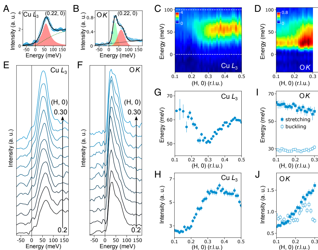
Fig. 2. Phonons in underdoped UD23. (A and B) Fitting examples of the inelastic excitation at the Cu L_3 - and O K edges. Fitting details are described in Materials and Methods . (C and D) Cu L_3 - and O K RIXS intensity maps as shown in Fig. 1 C and D with the fitted elastic peak subtracted. (E and F) Cu L_3 - and O K RIXS spectra after removing the fitted elastic peaks at selected momentum transfer values ranging from q_{||} = 0.2 to 0.3 r.l.u. along the (H, 0) direction. (G and H) The fitted dispersion and the integrated intensity of the bond-stretching phonon excitations at the Cu L_3 edge as a function of momentum. The phonon spectral weight is integrated within the energy window (0–100 meV) illustrated by the white dotted line in C. (I and J) The dispersion and integrated intensity of the bond-stretching phonon (the high-energy peak, filled markers) and the bond-buckling phonon (the low-energy peak, open markers) at the O K edge. The dispersion is extracted from the fitting. Phonon intensity is the area of the curve fitting each phonon mode.
