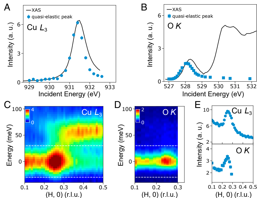
Fig. 1. CDW in underdoped UD23. (A and B) Solid black lines: Cu L_3 - and O K - edges XAS of UD23 sample collected with \sigma incoming polarization in normal incidence geometry (see the experimental setup in SI Appendix, Fig. S2). Blue circles (squares): Energy-dependent scattering intensities of the quasielastic peaks at the Cu L_3 -edge (O K edge) at q_{||} = 0.26 r.l.u. (0.25 r.l.u.). (C and D) RIXS intensity maps excited at the Cu L_3 resonance of 931.6 eV and the O K -edge hole-peak resonance of 528.4 eV as a function of energy and q_{||} along the (H, 0) direction. (E) Integrated intensity of the quasielastic peak, at the Cu L_3 - and O K edges, within an energy window ( \pm 30 meV) marked by the two white dashed lines in C and D.
