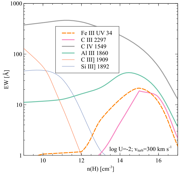
Figure 7. The effects of varying hydrogen density along the ridge of peak C IV emission strength, keeping the ionization parameter constant. C III \lambda 1909 and Si III \lambda 1892 produce very little emission above 10^{13} \text{ cm}^{-3} , where both Fe III UV34 and Al III \lambda 1860 are predicted to peak. C III \lambda 2297 is predicted to be strong above 10^{14} \text{ cm}^{-3} , but this line is not observed in quasar spectra.
