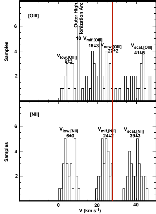
Figure 3. These histograms for the SE-Region show the frequency of line components in both [N II] and [O III] and are discussed in Section 2.2.1. The red line indicates the adopted velocity of the PDR (27.3 km s ^{-1} ).
