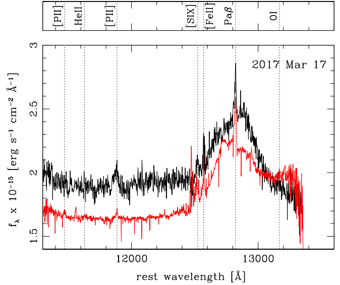
Figure 3. IRTF SpeX near-IR spectrum from 2017 March 17 (black) compared to the NIFS J band spectrum obtained by summing the flux in a 0.3'' \times 1.2'' aperture centered on the nucleus and oriented at the same position angle as the IRTF spectral aperture (red). The main emission lines are identified and labeled.
