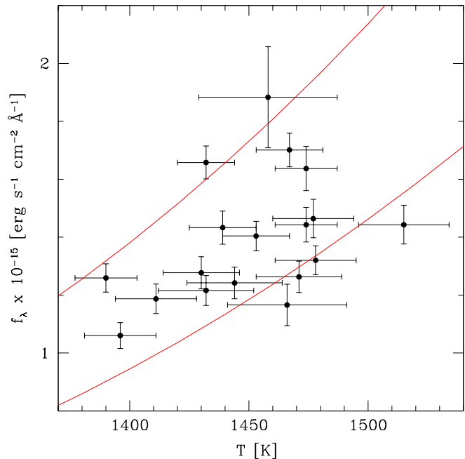
Figure 12. Flux in the wavelength region of 1.55 - 1.60 \mu\text{m} versus the temperature (for the blackbody case). We plot 1\sigma errors. The red curves show the expected relationship if the flux increase is solely due to a temperature increase. The spread in dust mass necessary to explain the flux difference between the two red curves is a factor of \sim 1.5 .
