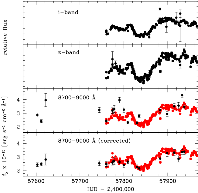
Figure 2. Top two panels: LCOGT i and z_s light-curves in relative flux units and not corrected for host galaxy contribution. Bottom two panels: IRTF SpeX near-IR spectral light-curve in the wavelength range 8700 – 9000 Å (black filled circles), both original and corrected using photometric correction factors based on the [S III] \lambda 9531 line, versus the z_s band light-curve corrected for a constant host galaxy contribution and scaled to match the IRTF spectral flux from 2017 March 17 (red filled circles).
