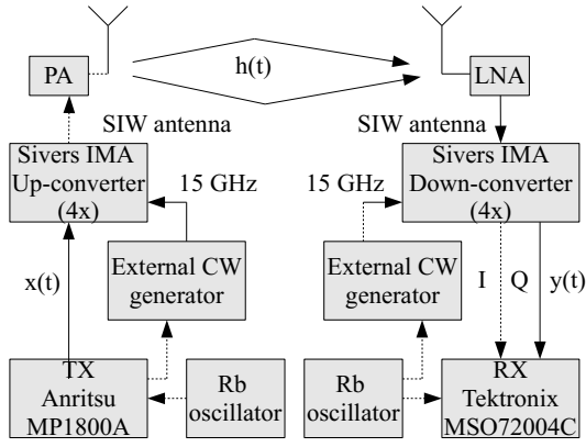
Fig. 3. Time-domain correlative channel sounder utilizing Golay sequences, omni-directional SIW antennas and local rubidium oscillators.
