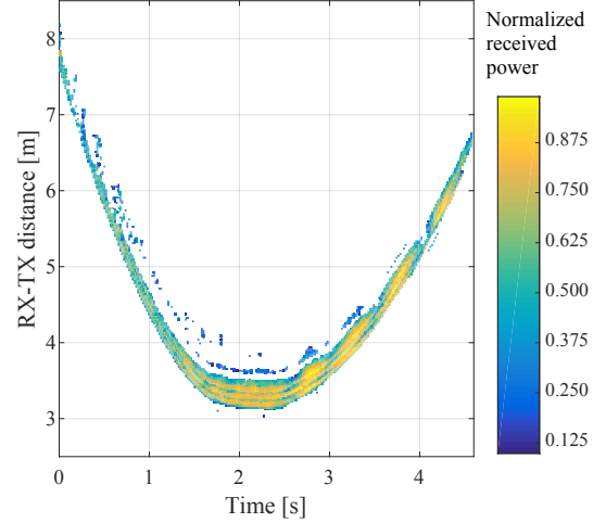
Fig. 4. Exemplary channel impulse recording of one pass of the vehicles. The measured data are thresholded, therefore the noise background is not depicted.
