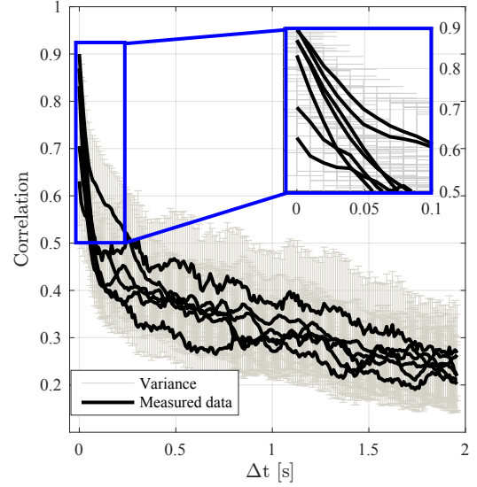
Fig. 6. Pearson correlation coefficient evaluation for several passes as a function of a correlation distance \Delta t .
