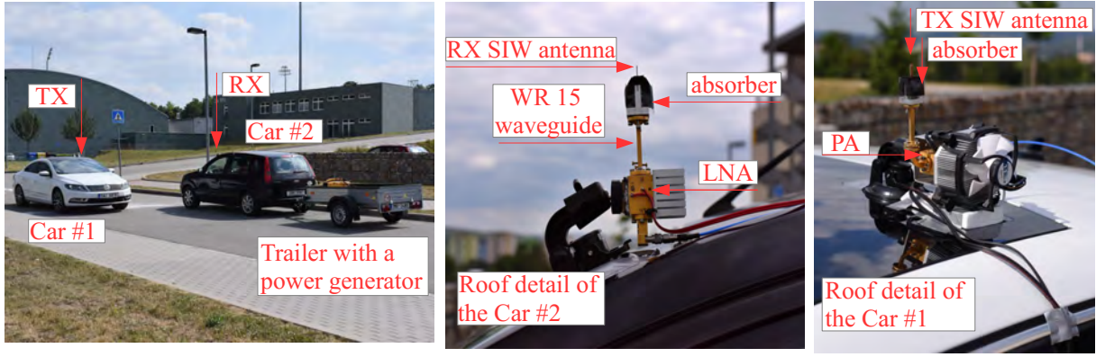
Fig. 2. Photographs taken during the measurement campaign. Two measurement vehicles, Car #1 (with a battery pack in the trunk) and Car #2 (with a 2 kW gas-powered generator on the depicted trailer) at their approximate meeting point. Picture of TX and RX mounting including PA and LNA installation detail.
