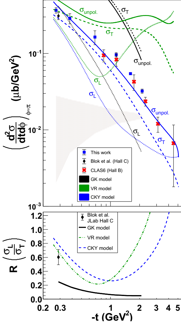
FIG. 4. (Color Online) ( top panel ) Unpolarized cross sections ( \frac{d^2\sigma}{dt d\phi} ) vs -t , as the blue squares with error bars representing total random errors (statistical and random systematic added in quadrature) of this work. The systematic uncertainties are represented with shaded band. The data point represented with black diamond at lower -t value is Blok et al. [4] unpolarized cross section result, while the red crosses are the kinematically corrected results from JLab Hall B [10]. The results from the Regge amplitude based VR [15], CKY [12] and GPD-based GK [16, 17] models are also shown in green, blue and black solid lines, respectively. Additionally shown are the model longitudinal (transverse) contributions to the unpolarized cross sections by dotted (dashed) lines. ( bottom panel ) The ratio ( R = \frac{\sigma_L}{\sigma_T} ) vs -t . The only L/T separated existing data, from F_{\pi-2} Hall C [4], are represented by the black diamond. The green dot-dashed, blue dashed and black solid lines represent the VR, CKY and GK models, respectively. The model predictions diverge considerably in the region -t > 1 \text{ GeV}^2 .
