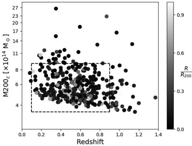
Figure 1. The mass redshift distribution of 368 SPT clusters imaged with DES Y3 data. The dashed box corresponds to limits applied to the SPT-SZ sample to select our sample. In light grey clusters with larger BCG to SZ centroid offset ( D_{\text{BCG-SZ}} ) while the dark points correspond to systems with lower D_{\text{BCG-SZ}} .
