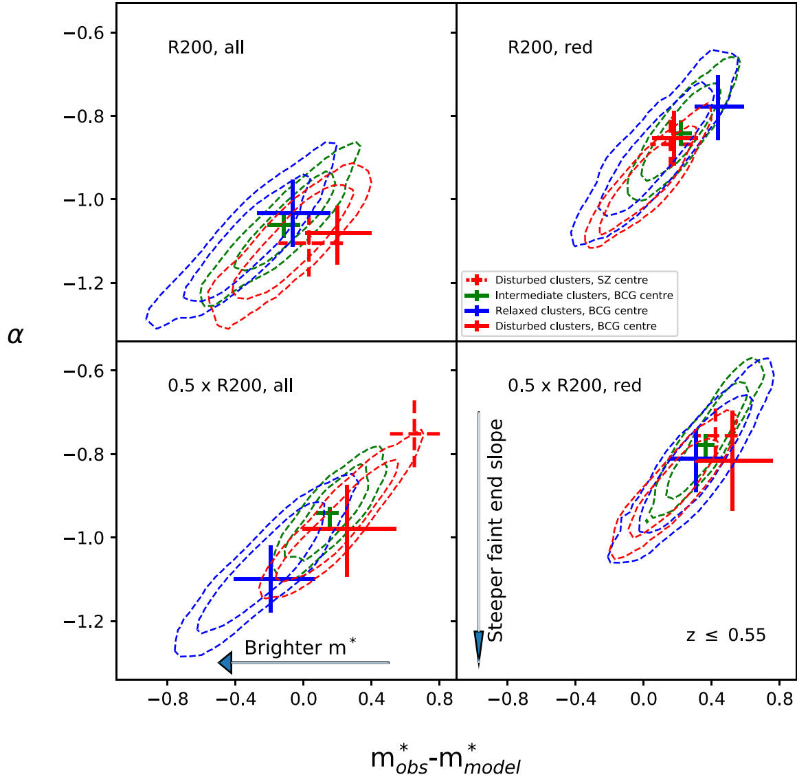
Figure 11. \alpha - m^*(m_{\text{obs}}^* - m_{\text{model}}^*) for cluster galaxies (all) and RS galaxies (red), within 1 and 0.5 r_{200} , at z \leq 0.55 . We obtain m_{\text{obs}}^* by fitting the data, while m_{\text{model}}^* corresponds to the model as discussed in Section 2.4. Solid red crosses represent disturbed clusters using the BCG as a centre (26 clusters), dash red crosses represent disturbed clusters using the SZ centroid as a centre, blue crosses correspond to the relaxed sample (16 clusters) while green crosses correspond to the intermediate sample (see Section 4.1.3 for details; 111 clusters), both using the BCG as a centre. Dashed red/blue contours correspond to 68 per cent and 90 per cent of the fits, when the centre is randomized 600 times within 0.4-1 r_{200} of the SZ centre, for the disturbed/relaxed sample. Green contours correspond to 68 per cent and 90 per cent of the fits, obtained by stacking 26 randomly selected clusters from the intermediate cluster sample, using the BCG as a centre 600 times. At this redshift range all cluster populations seems to occupy a very similar \alpha - m^* parameter space.
