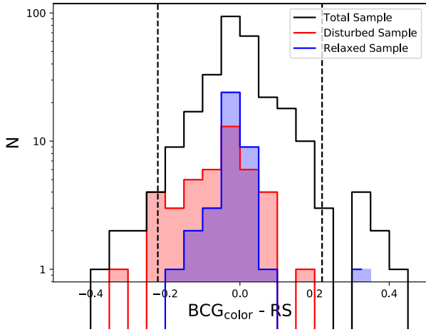
Figure 6. BCG colour for the total, the relaxed, and the disturbed cluster samples with respect to the RS (as defined in Section 2.4). The BCG colours, and m^* , are estimated depending on the cluster redshift; g - r at z < 0.35 , r - i at z < 0.7 , and i - z at z > 0.7 . Vertical lines are at \pm 0.22 mag, corresponding to our 3\sigma RS width (López-Cruz et al. 2004).
