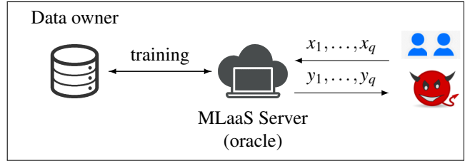
Figure 1: Model extraction can be envisioned as active learning. A data owner, with the help of a MLaaS server, trains a model f^* on its data. The proprietary model is stored by the server, which also answers to queries from users ( i.e. , y_i = f^*(x_i) ). In a model extraction attack, a dishonest user tries to exploit this interface to “steal” f^* in the same way as a learner uses answer from a machine-learning oracle in order to learn f^* .
