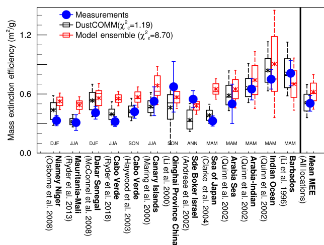
Figure 8. Comparison of measurements (blue dots) of dust MEEs ( \text{m}^2 \text{g}^{-1} ) against column-integrated DustCOMM (black bars) and model ensemble (red bars) estimates. Vertical bars on the measurements represent reported uncertainty. For the DustCOMM and model ensemble estimates, the black and red boxes show 1 standard error, whereas the vertical dotted lines show the 95 % confidence interval; the middle horizontal bar and star show the median and mean values, respectively. The DustCOMM and model ensemble values are season-averaged values corresponding to the observation time period (see Table 2 for details). These seasons are labelled DJF – Dec–Feb, MAM – Mar–May, JJA – Jun–Jul, and SON – Sep–Nov; ANN represents an annually averaged value. The model ensemble MEE is calculated from the ratio between individual model dust aerosol optical depth and the dust mass loading, while the DustCOMM MEE is calculated using the constrained dust size distributions and single-particle extinction efficiency that takes into account the asphericity of dust aerosols. \chi^2_\epsilon is the reduced chi-squared value (Eq. 10b) and quantifies the performance of a model in representing observations (e.g. Andrae et al., 2010).
