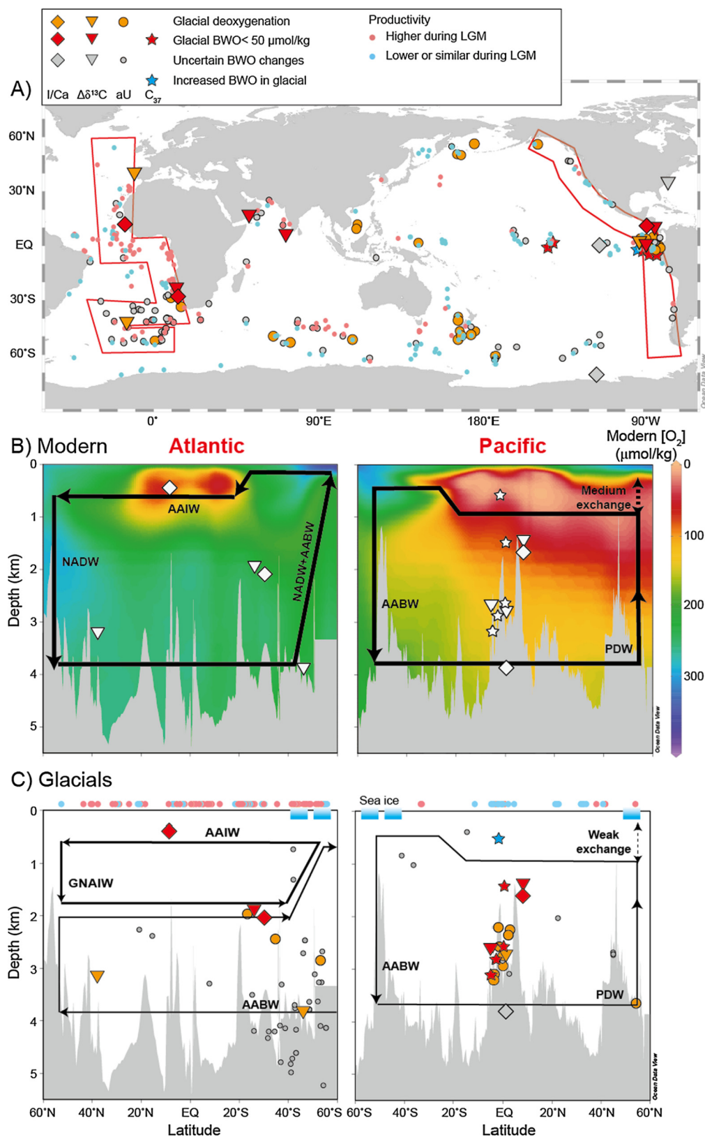
Fig. 5. Global compilation of benthic I/Ca, \Delta\delta^{13}\text{C} , \text{C}_{37} alkenones, and aU proxy records. (A) Map view, (B) modern and (C) glacial transects through the Atlantic and Pacific Oceans. Red symbols highlight sites with glacial deoxygenation and glacial BWO < 50 \mu\text{mol/kg} , as estimated from I/Ca < 3 \mu\text{mol/mol} , or an order-of-magnitude higher of \text{C}_{37} alkenones, or calculated from \Delta\delta^{13}\text{C} . “Uncertain” refers to sites without sufficient Holocene and/or glacial samples for I/Ca or \Delta\delta^{13}\text{C} analyses and factors other than BWO hampering the interpretation of aU as BWO proxy, respectively. Note that the \Delta\delta^{13}\text{C} calculated from C. kullenbergi at Sub-Antarctic Atlantic site MD07-3076Q (44.15°S, 14.23°W, 3.8 km) (Gottschalk et al., 2016a) has been re-calculated (Gottschalk et al., 2016b), because the calibration was only applicable for \delta^{13}\text{C}_{\text{C. wuellerstorfi}} . The productivity changes at the LGM relative to the late Holocene are adapted from Costa et al. (2017); Kohfeld et al. (2005). The ocean circulation in panel B and C is adapted from Du et al. (2018); Sigman et al. (2010). NADW: North Atlantic Deep Water; AABW: Antarctic Bottom Water; AAIW: Antarctic Intermediate Water; GNAIW: Glacial North Atlantic Intermediate Water; PDW: Pacific Deep Water.
