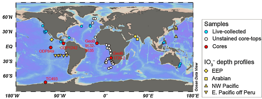
Fig. 1. Core and sample locations (EEP: Eastern Equatorial Pacific).
