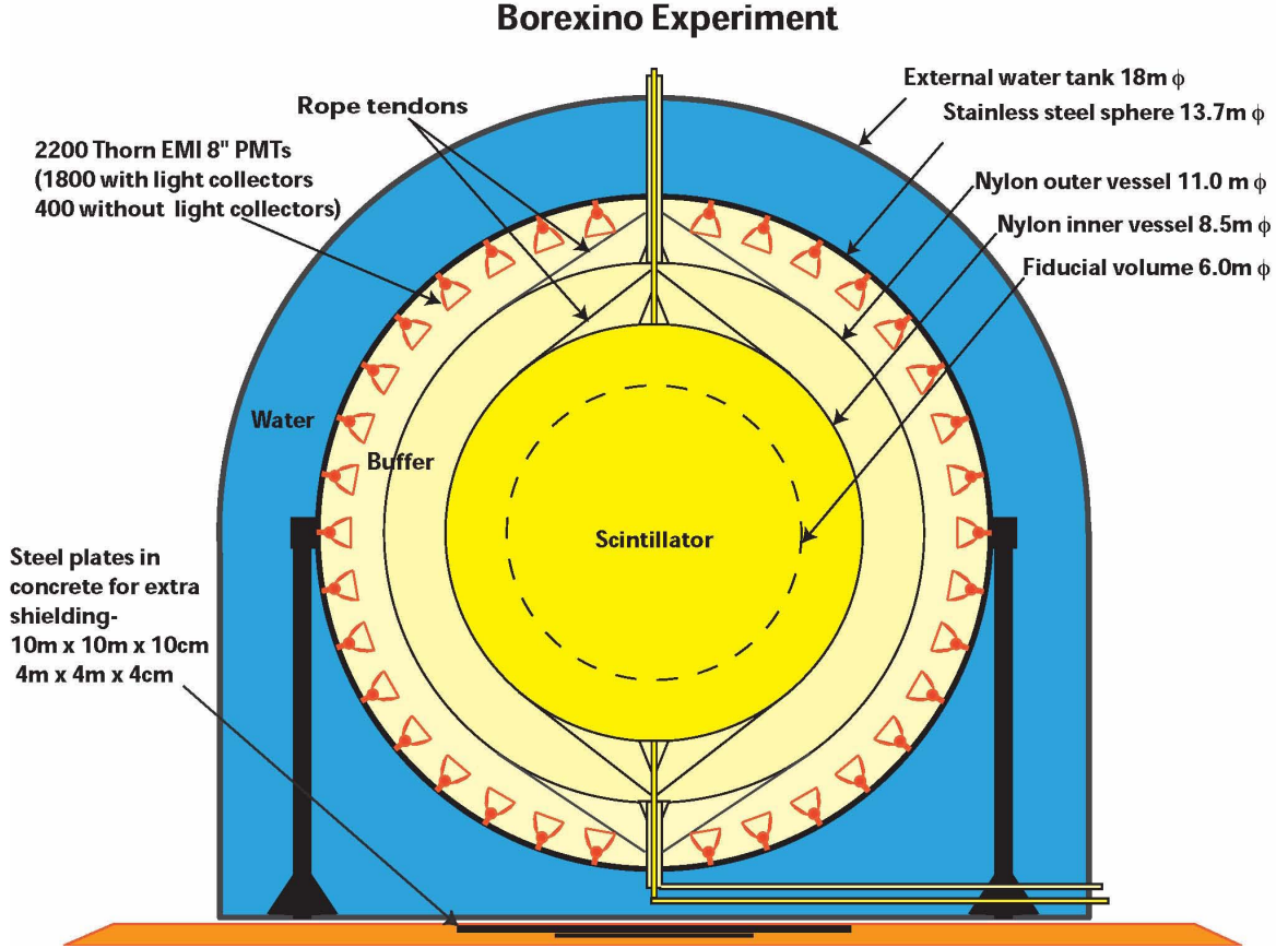
Figure 1. Schematic drawing of the Borexino detector.
