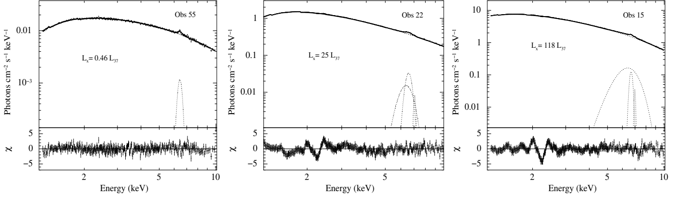
Figure 3. The 1.2–10 keV energy spectrum of Swift J0243.6+6124 with NICER at three representative luminosities after fitting with an absorbed cutoff power-law model plus Gaussian components (top panel). A single narrow line at \approx 6.4 keV was required at the lower luminosity (left; Obs 55). Two emission lines were clearly detected in the Fe-band at higher luminosity (middle; Obs 22). The energy spectrum at the super-Eddington state is described using an absorbed cutoff power-law model with three line components (right; Obs 15). Spectral residuals corresponding to the best-fitting models are shown in the bottom panels. The feature observed in the 2–3 keV range of the residuals (middle and right panels) is possibly instrumental in origin.
