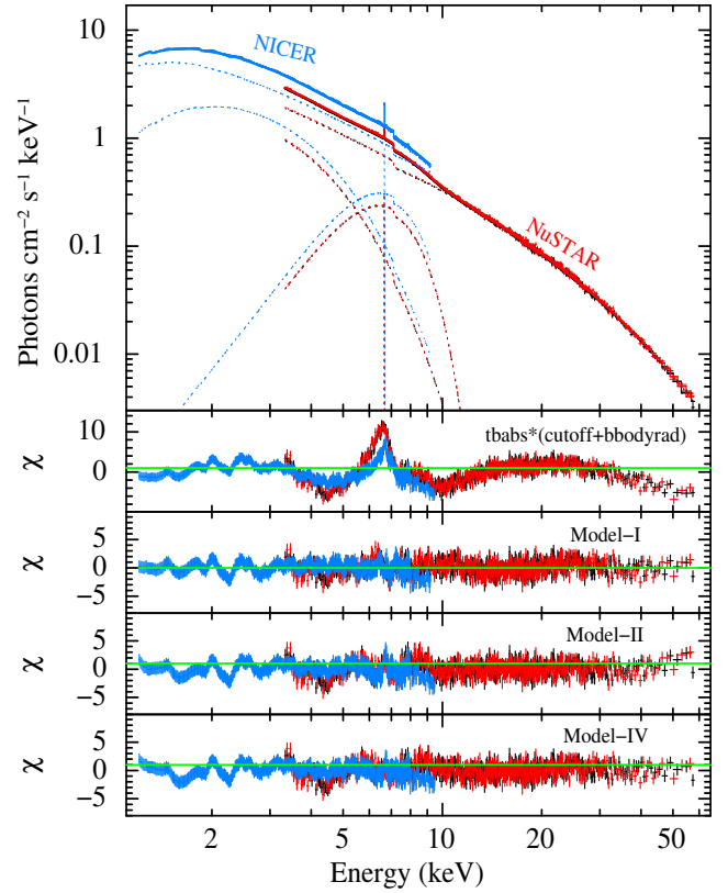
Figure 7. The 1.2–79 keV energy spectrum of Swift J0243.6+6124 obtained from quasi-simultaneous NICER and NuSTAR observations at the peak of the 2017 outburst along with (top and middle panels) the best-fit model comprising a cutoff power-law continuum with a blackbody component, three Gaussian functions, and an edge feature (Model-I). Spectral residuals corresponding to additional models, TBABS*(CUTOFF+BBODYRAD), Model-II: TBABS*(GSMOOTH*COPLREFL+HECUT+BBODYRAD), and Model-IV: TBABS*(RELXILL+CUTOFF+BBODYRAD) are shown in the remaining panels. The cross normalization constant between NICER and NuSTAR is 1.3 for the brightest observation of the source. The value is obtained with respect to the NuSTAR /FPMA detector.
