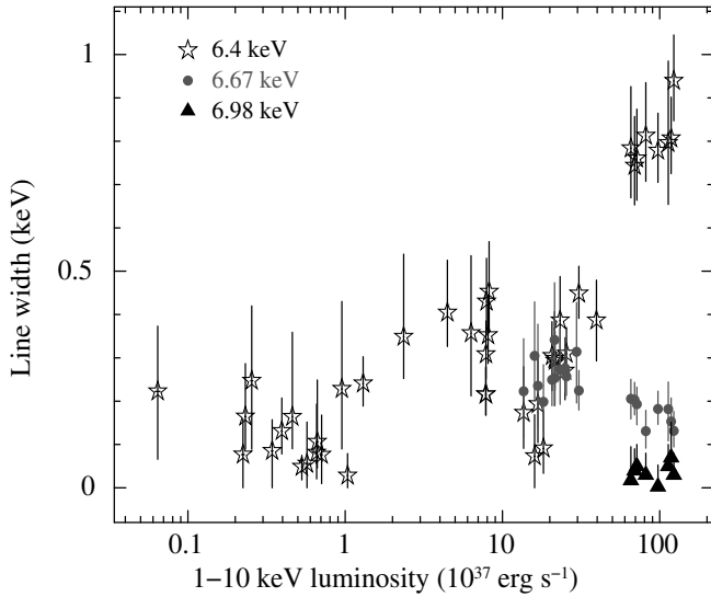
Figure 4. The luminosity evolution of line width for 6.4, 6.67, and 6.98 keV emission components during the outburst.
