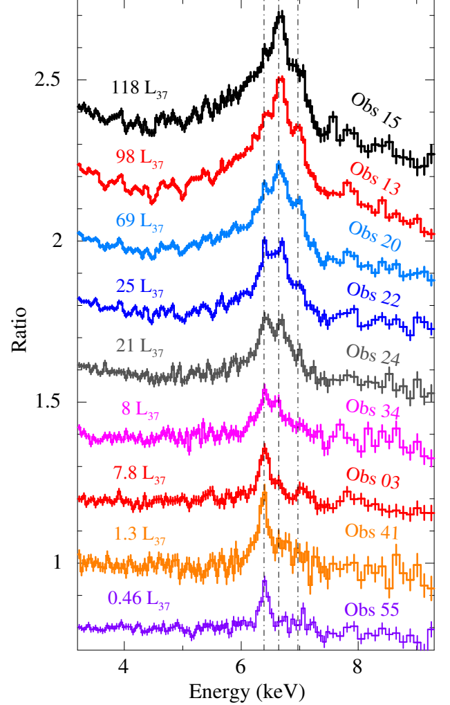
Figure 2. Ratio of NICER data to the continuum model (scaled arbitrarily) obtained by fitting 1.2–10 keV energy spectra of Swift J0243.6+6124 with an absorbed cutoff power-law model. These are arranged in order of increasing luminosity. L_{37} stands for unabsorbed luminosity in units of 10^{37} erg s -1 . Observation IDs (10503901xx) are also shown as labels. Three emission lines in the 6–7 keV range are detected at 6.4, 6.67, and 6.98 keV energies (vertical dash-dot lines).
