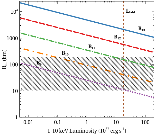
Figure 8. Evolution of the magnetospheric radius ( R_m ) with luminosity for a range of dipole magnetic fields. Here, B_n denotes the field strength in units of 10^n G. The shaded area presents a zone up to a distance of \approx 200 km from a canonical neutron star, allowing a relativistic iron line profile from the emitting medium due to gravitational effects. We observed a broad Fe-line clearly from Swift J0243.6+6124 in the super-Eddington regime. If the line originates from the disk, a possible solution of the pulsar B-field can be obtained as an order of 10^{11} G.
