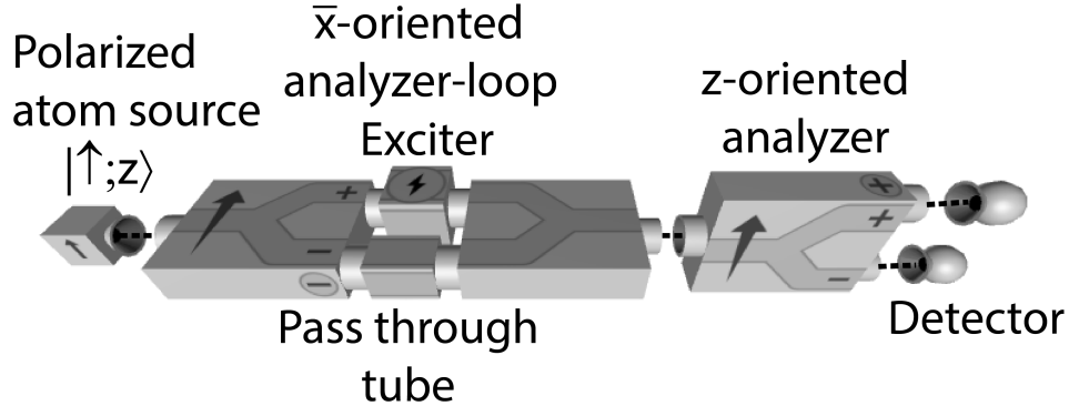
FIG. 7. “Un erased” version of a quantum eraser “experiment” with an analyzer loop-exciter (exciting on the + path of the \bar{x} -oriented analyzer loop) and a z -oriented analyzer to detect the spin projection of the atoms at the end of the experiment.
