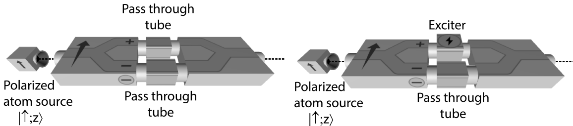
FIG. 6. (Left) Analyzer loop oriented along the \bar{x} direction with pass-through tubes, which allow the beam to pass without blocking a path or detecting if an atom went through a path. The source produces polarized |\uparrow; z\rangle atoms. (Right) Analyzer loop with an exciter on the + branch and a pass through tube on the - branch. The dotted line shows the path the atoms take through the device.
