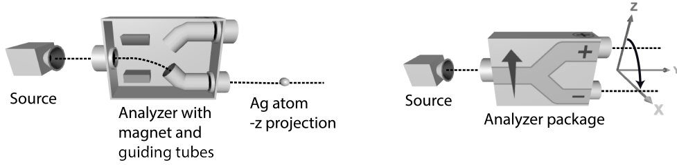
FIG. 2. Schematic of the quantum Stern-Gerlach experiment with silver atoms, which produces only two deflections. Both images start with an unpolarized source of silver atoms on the left. The packaging with an inhomogeneous magnet and “guiding tubes” on the left image is covered with a schematic annotation creating the Stern-Gerlach analyzer in the right image, which also illustrates the coordinate system used to describe the orientation of the analyzer (here the orientation corresponds to an angle in the x - z plane as indicated by the curved arrow). The dotted lines indicate the path an atom with a negative projection takes through the device (left) and schematically shows the two possible paths that an initially unpolarized atom can take (right).
