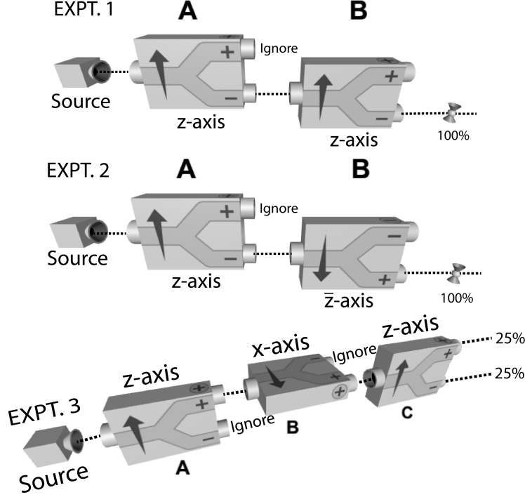
FIG. 3. Three different “experiments” with Stern-Gerlach analyzers all starting from an unpolarized source. (Top) Experiment 1, measure on the z -axis (A), capture all from the - exit and then measure on the z -axis again (B). This “experiment” shows that measurements on an analyzer are reproducible. (Middle) Experiment 2, measure on the z -axis (A), capture all from the - exit and then measure on the \bar{z} -axis (B). This “experiment” shows that a positive projection on one axis is a negative projection on the inverse axis and vice versa . (Bottom) Experiment 3, measure on the z -axis (A), capture all from the + exit, measure on x -axis (B), capture all from the + exit, and then measure on z -axis again (C). Since we only input atoms with a positive z -axis projection into (B), one might expect that they will all emerge with a positive projection on the z -axis from (C), but we find they are equally likely to emerge with a positive or negative projection on the z -axis, because the angular momentum operators in different Cartesian directions are incompatible operators, and the atom can have a definite projection on only one axis at any given moment.
