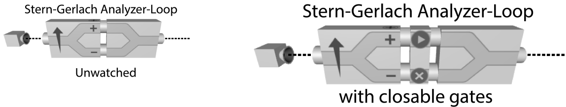
FIG. 4. (Left) Schematic of an analyzer loop, which can be thought of as two oppositely oriented Stern-Gerlach analyzers attached back-to-back. If no measurement is made, then the analyzer loop does not alter the quantum state of the atom and it emerges with the same state it entered. If one of the paths is blocked, the atom emerges with the state given by the path that is not blocked (and the probability to emerge is determined by the state the atom had when it entered). (Right) a Stern-Gerlach analyzer loop with a flow-through gate. The gate can be independently controlled to block zero, one, or two branches of the analyzer loop. The pictured flow-through gate is configured to block the lower branch of the analyzer loop (as indicated by the \times ). Blocking one path is a measurement. For example, if the atom entered in a state with a positive projection along the x -axis, half of the atoms would be blocked, and half would exit in the |\uparrow; z\rangle state. The dotted lines show the paths the atoms take through the devices.
