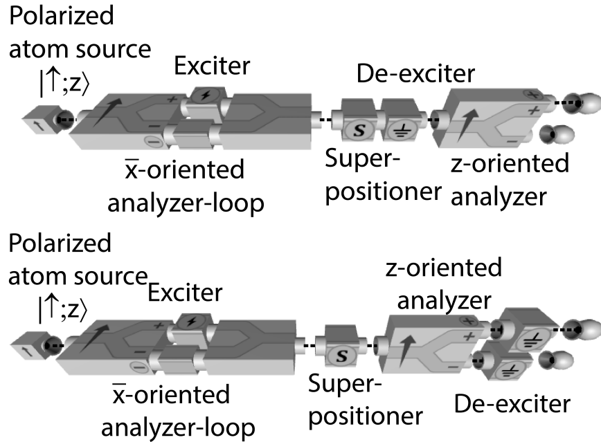
FIG. 8. Fully erased quantum eraser “experiment” with the eraser elements (superpositioner and de-exciter) either both positioned before the final analyzer (top) or one before and one after (bottom). In the second case, the de-exciter can be placed as far from the analyzer as desired. Note how in this latter case, atoms emerge from both exits of the z -oriented analyzer, but only those that are in the |\uparrow\rangle \otimes |GS\rangle state can pass through the de-exciter and be detected. The delayed choice corresponds to whether the de-exciter is inserted or not; we have pictured the case where it is inserted.
