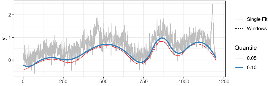
FIG. 4. Trend fit with our ADMM algorithm with three windows (converged in seven iterations), compared to trend from simultaneous fit.
