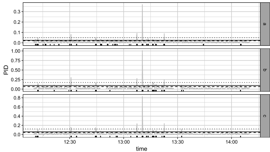
FIG. 12. Rugplot showing locations of signal after baseline removal using the detrendr estimate of 5th quantile. Horizontal dashed lines represent the thresholds calculated using the 90th, 95th and 99th quantiles of the detrended data. The 95th quantile (solid line) was used to classify the signal shown as vertical lines at the bottom of the plot.
