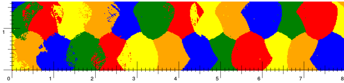
(b) Coloring using hexagons with edge length 0.01 and height 1.66
