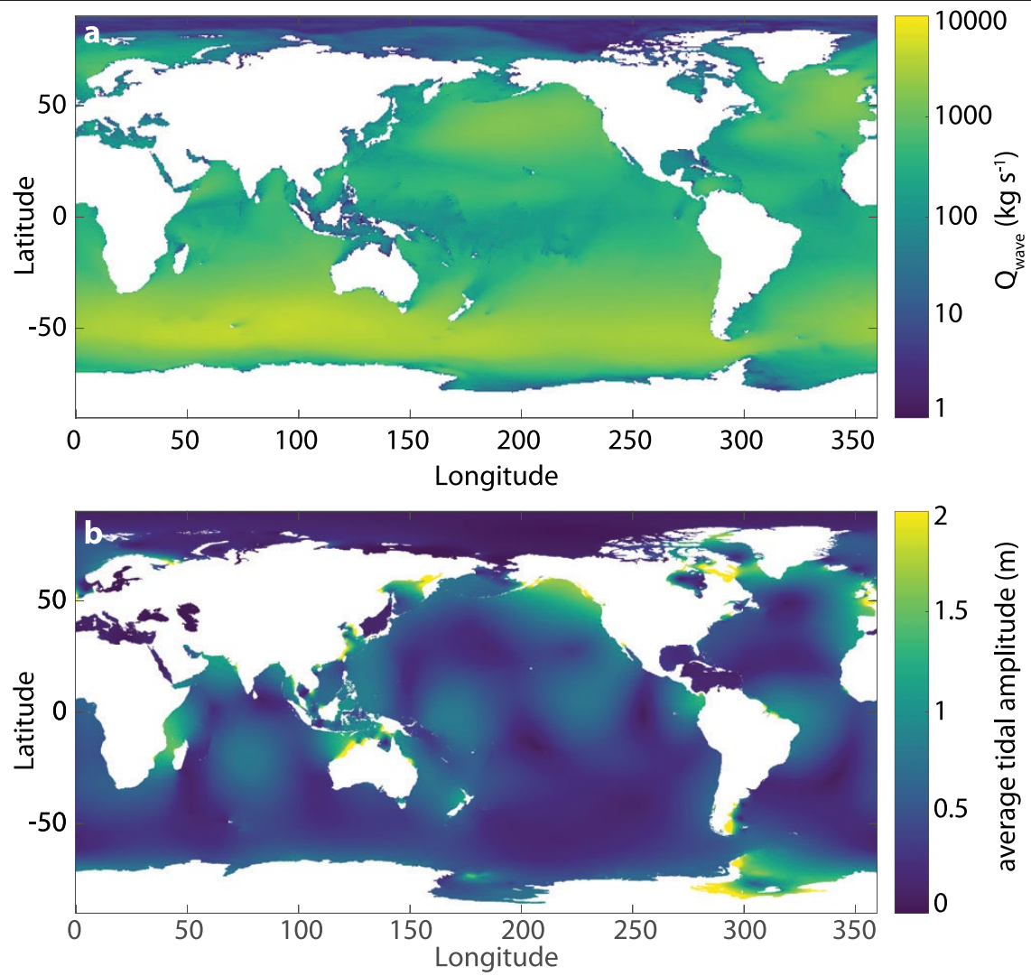
Extended Data Fig. 4 | Characterization of data used for wave- and tide-driven deltaic sediment flux. a, Global maximum potential alongshore sediment transport ( Q_{\text{wave}} ) based on the WaveWatch 30-year hindcast data 47 . b, Global estimate of mean tidal amplitude based on the OSU TOPEX data 30 .
