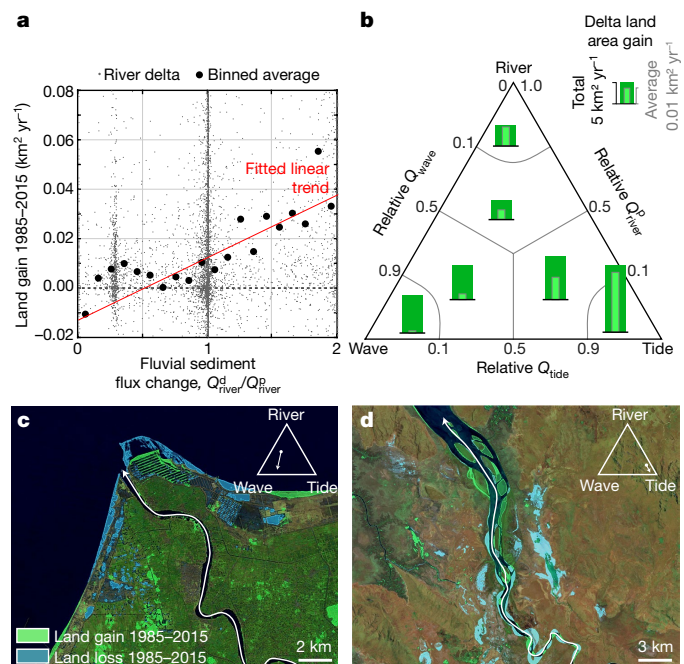
Fig. 3 | Rates and drivers of delta land area change over the period 1985–2015.
