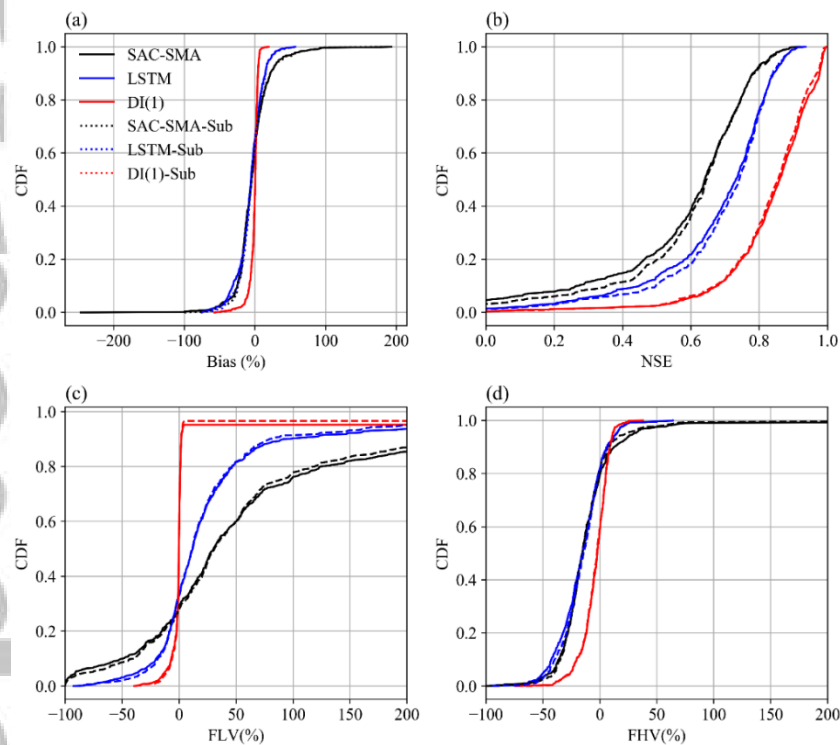
Figure 4. Comparison of the cumulative density functions (CDF) for the DL models and the SAC-SMA hydrologic model. The “-Sub” suffix refers to the 531-basin subset used in previous studies, for comparison. FLV: The percent bias of low flow regime (bottom 30%); FHV: The percent bias of high flow regime (top 2%). The SAC-SMA model was calibrated from 1980-Oct-01 to 1995-Sep-30 and was evaluated from 1995-Oct-01 to 2005-Sep-30. LSTM and DI(1) were trained from 1985-Oct-01 to 1995-Sep-30, and the metrics were evaluated from 1995-Oct-01 to 2005-Sep-30. The CDF of FLV does not reach 1.0 because some basins have all zero flow observations for the 30% low flow interval, the percent bias can be infinite, and thus the x-axis cannot cover those basins. We set its x-axis to the same range as FHV.
