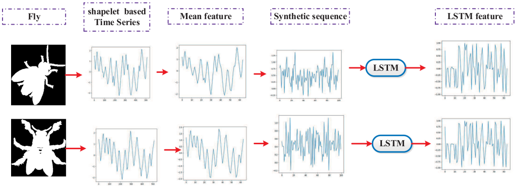
Fig. 11. Comparisons between original time mean features vs. LSTM features learned from GeLSTM converted sentence for same class images with rotation (“fly”).
