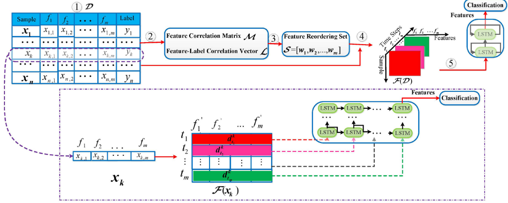
Fig. 5. An overview of the proposed GeLSTM which generalizes LSTM for deep learning from generic data. For a generic dataset represented in instance-feature tabular format in ①, GeLSTM first calculates feature-feature correlation matrix and feature-label correlation vector ②. Next, GeLSTM builds a feature reordering set ③, and converts the original two-dimensional data dataset into three-dimensional tensor ④ which is fed into LSTM module ⑤ for learning features for classification. Lower panel (dashed-line box) shows the conversion of instance \mathbf{x}_k into a synthetic sentence format with m words \mathcal{F}(\mathbf{x}_k) = [d_{t_1}^k, d_{t_2}^k, \dots, d_{t_m}^k] . The i^{th} word d_{t_i}^k is fed into the unfolded LSTM unit at time step t_i .
