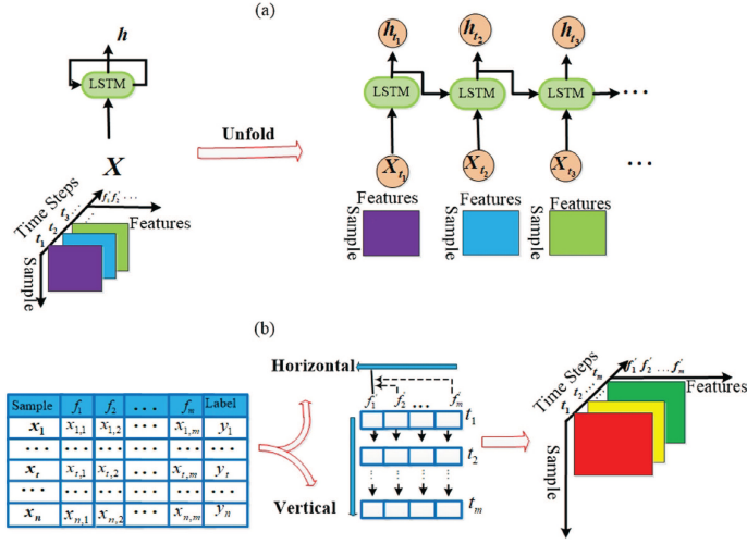
Fig. 4. (a): A conceptual view of the LSTM network. Left panel shows an LSTM network with three-dimensional tensor input (i.e., [samples, time steps, features]), and the right panel shows the unfolded LSTM where each LSTM unit corresponds to one time point; and (b) a conceptual review of the proposed GeLSTM which converts a generic dataset (left panel) into three dimensional tensor input (right panel) using horizontal-vertical feature alignment (middle panel).
