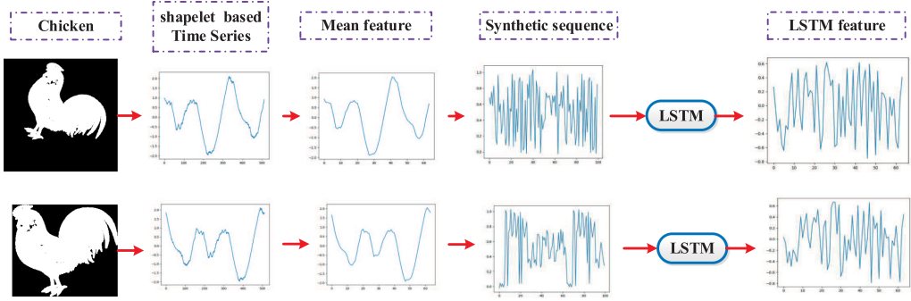
Fig. 12. Comparisons between original time mean features vs. LSTM features learned from GeLSTM converted sentences for same class images with rotation (“chicken”). The results show that mean features are sensitive to rotation, whereas LSTM features learned from GeLSTM converged sentences is robust to the rotation, and both images show similar LSTM features.
