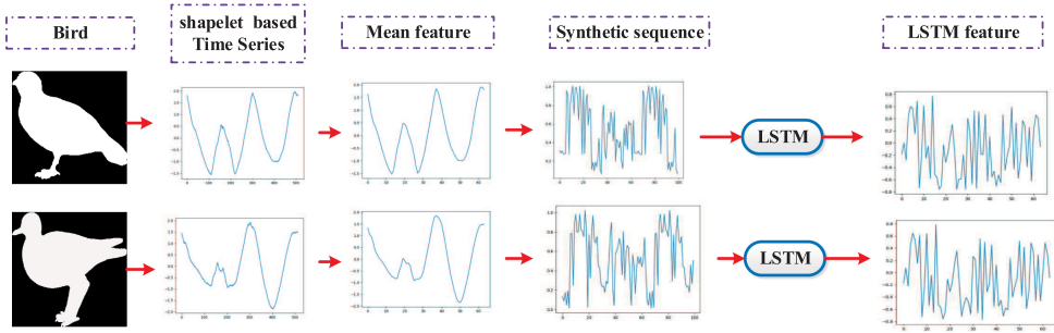
Fig. 10. Comparisons between original time mean features vs. LSTM features learned from GeLSTM converted sentences for same class images with rotation (“bird”).
