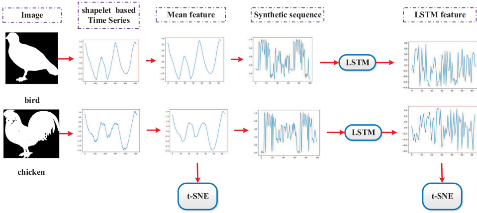
Fig. 8. Comparisons between original time mean features vs. LSTM features learned from GeLSTM converted sentence for the instances from different classes (“bird” vs. “chicken”).
