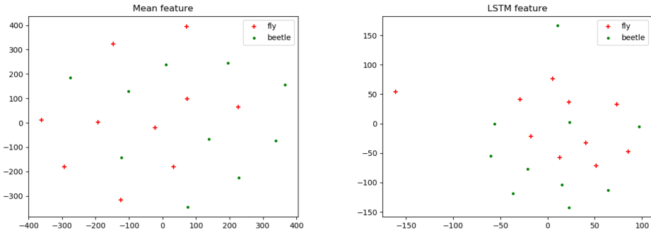
Fig. 13. Comparisons between original features (mean) vs. GeLSTM learned LSTM features (“Beetle” vs. “Fly”). Instances are color-and-shape coded, according to their labels. The plot on the left panel shows the instances with respect to the original features, and the plot on the right panel shows the GeLSTM learned LSTM features. Both plots are produced using t -SNE feature visualization tool [52].
