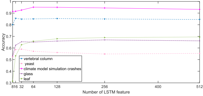
Fig. 6. Accuracy comparisons w.r.t. different number of LSTM output features, where the x -axis denotes the number of learned features, varying from 8 to 512, and the y -axis denotes the accuracy reported in decimal numbers.
