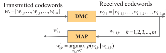
Fig. 15. A conceptual view of communication system considering the discrete memoryless channel (DMC) and the maximum a posterior probability (MAP) decoder: The transmitted codewords \mathbf{w}_t \in C passes through the DMC, and DMC outputs the received codewords \mathbf{w}_{i-1} . By utilizing the likely transmitted codeword w_{i,k} and the received codeword w_{i-1,k} , the MAP decoder estimates the k^{th} transmitted codeword (the estimated result is denoted by w'_{t,k} ).
