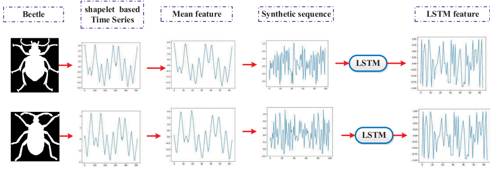
Fig. 9. Comparisons between original time mean features vs. LSTM features learned from GeLSTM converted sentences for the instances without image rotation from the same classes (“beetle”).
