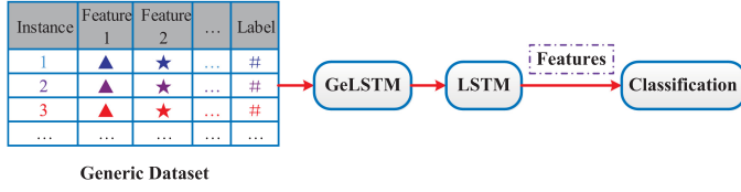
Fig. 3. Typical workflow of utilizing the proposed GeLSTM framework to make LSTM available for generic data classification tasks.
