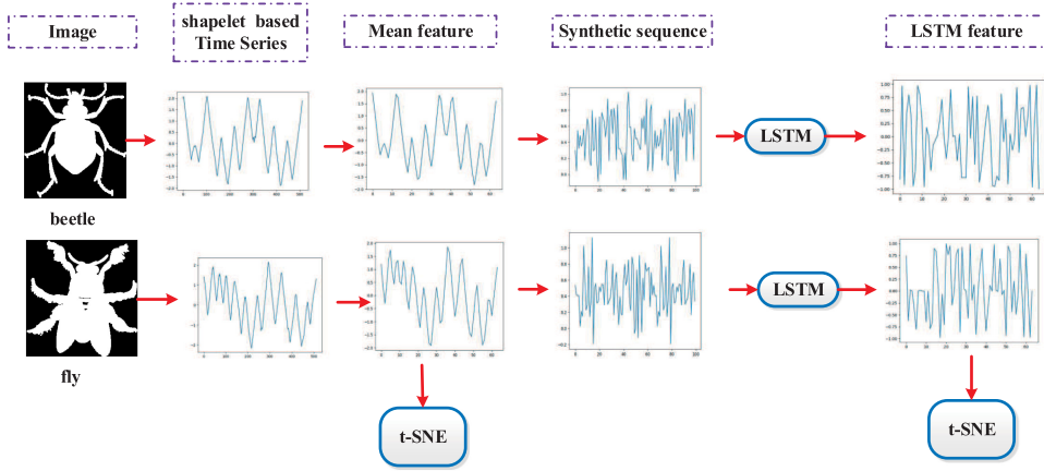
Fig. 7. Comparisons between original time mean features vs. LSTM features learned from GeLSTM converted sentence for the instances from different classes (“beetle” vs. “fly”). The data on time series curve is obtained from UCR time series archive [14] which are mapped from the outline of the image, and then extract the 64-dimensional mean features from the time series to obtain the data on the mean feature curve. After that, by applying GeLSTM method to convert mean represented instances, data on the synthetic sequence curve is available, which are further fed into the LSTM model to learn LSTM feature. Finally, we employ the t -SNE tool [52] to make a comparison between the original mean features and the LSTM learned features to further explain the benefits of our proposed GeLSTM method.
