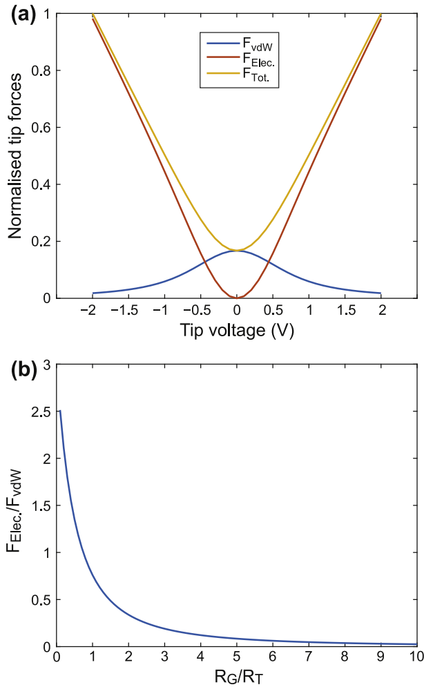
Fig. 4. Calculated van der Waals and electrostatic forces between the tip and graphene, modelled for the suspended few-layer ( n = 6 ) graphene case (a) as a function of voltage just before the graphene discontinuously deflects up to the probe on approach at point B in schematic, and (b) the ratio of the two forces once the graphene is 'attached' to the tip (region C in schematic) at bias V = \pm 2 V as a function of the graphene to tunneling resistance ratio. (A colour version of this figure can be viewed online.)
