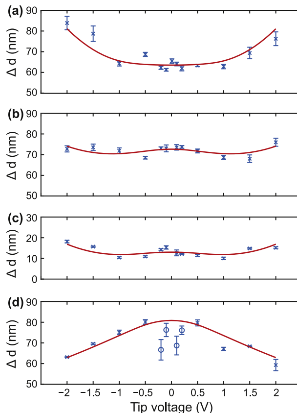
Fig. 3. Mean graphene displacement from the initial upward deflection to the point at which the graphene fully detaches from the probe ( \Delta d ) with standard error: (a) few-layer ( n = 6 ) supported (b) few-layer suspended (c) multi-layer ( n=8 ) supported and (d) multi-layer suspended. An example modelled response is overlaid for each dataset as solid lines. (A colour version of this figure can be viewed online.)
