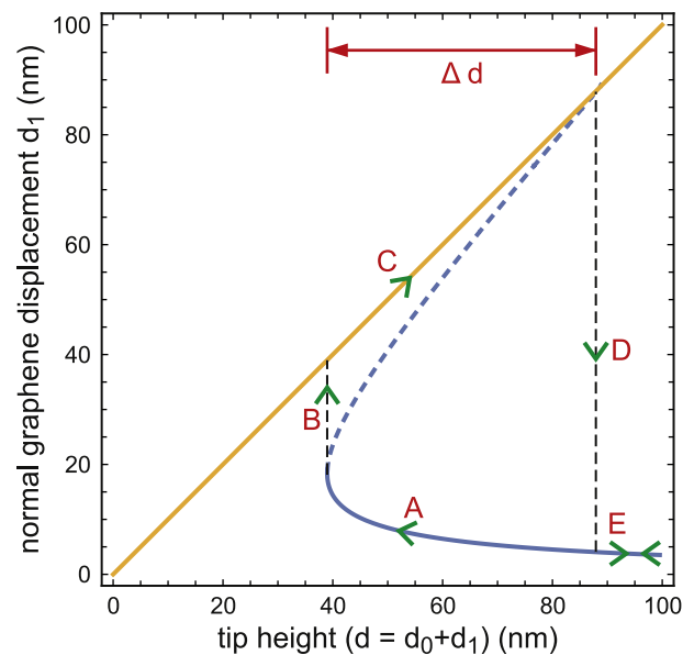
Fig. 2. Example of a hysteresis response from the force-balance model showing the normal displacement of the graphene d_1 against the tip–graphene distance at rest, d . Labels match the experimental data in Fig. 1. (A colour version of this figure can be viewed online.)
