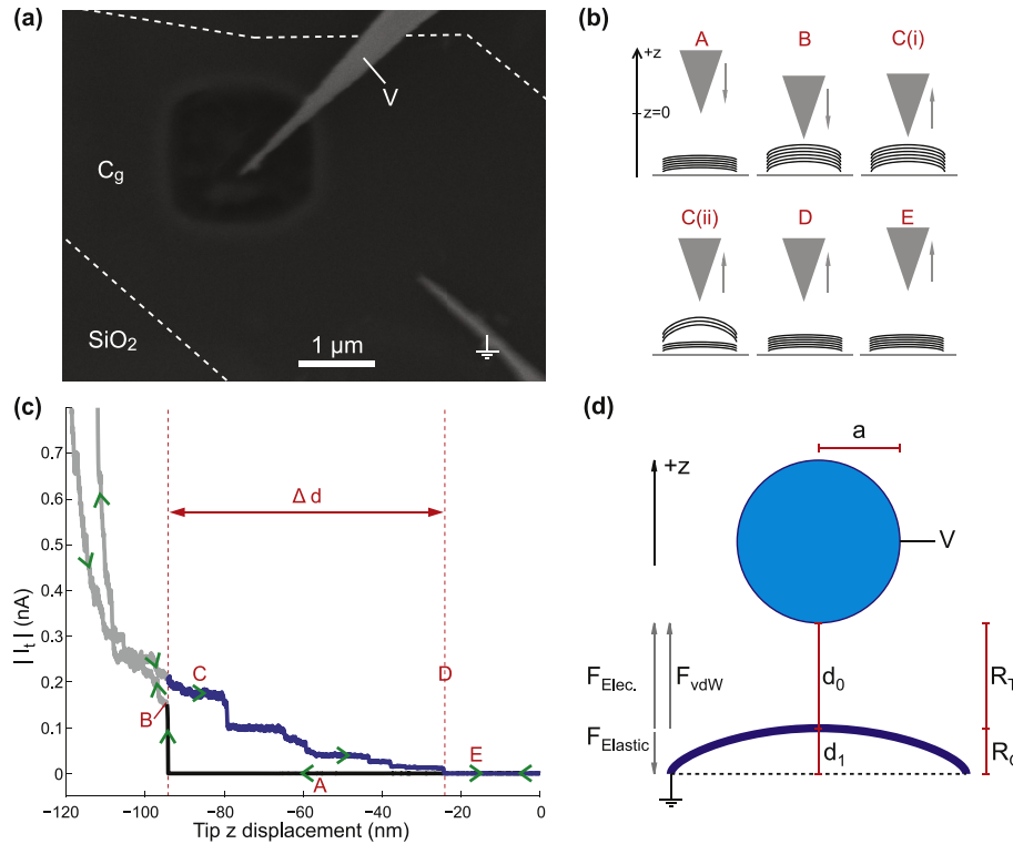
Fig. 1. (a) SEM image of two tips positioned over few-layer ( n = 6 ) graphene on SiO 2 . Bottom right tip at ground and in contact with the graphene, upper tip just out of tunneling contact with the portion of the graphene suspended over a hole in the substrate. Dashed lines mark the boundary of the graphene flake on the SiO 2 substrate. (b) Schematic diagram of the approach and retraction phases with matching labels. (c) example approach–retraction STM measurement truncated at 0.8 nA for V_{tip} = +0.01 V. (d) A schematic of the model with matching variables. (A colour version of this figure can be viewed online.)
