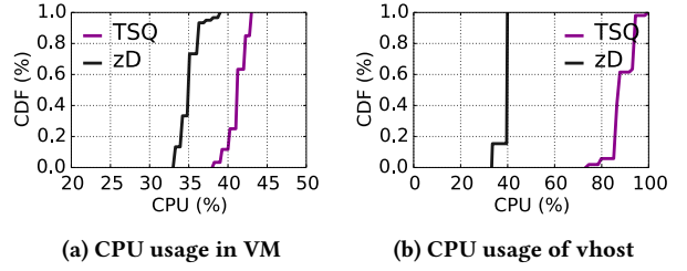
Figure 4: zD reduces CPU usage in both VM and the physical machine compared to standard kernel implementation for TSQ (pfifo).
