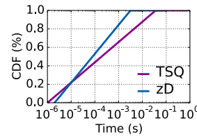
Figure 15: CDF of flow RTT with hypervisor-only zD.
