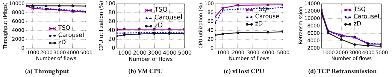
Figure 13: Compared with Carousel, zD achieves higher throughput, lower VM CPU usage, lower vHost CPU usage, and fewer TCP retransmissions
