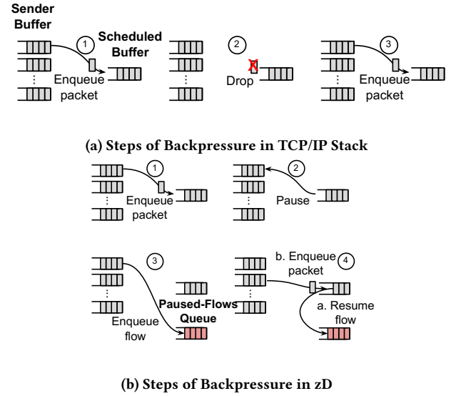
Figure 7: Illustration of different backpressure steps.
