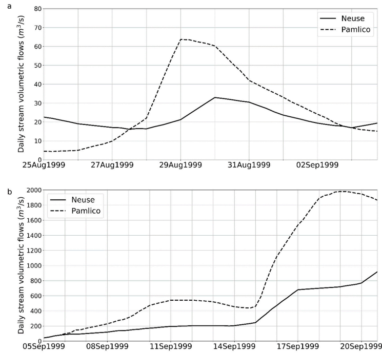
Figure 6. Daily stream volumetric flows in the Tar-Pamlico and Neuse Rivers for the period of (a) August 25 to September 04 and (b) September 04 to September 20, 1999.
