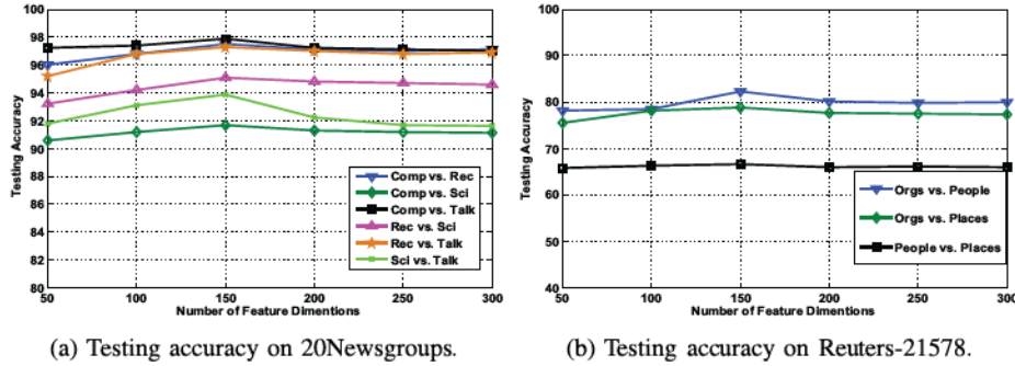
Fig. 4: Classification results with different feature dimensions.
