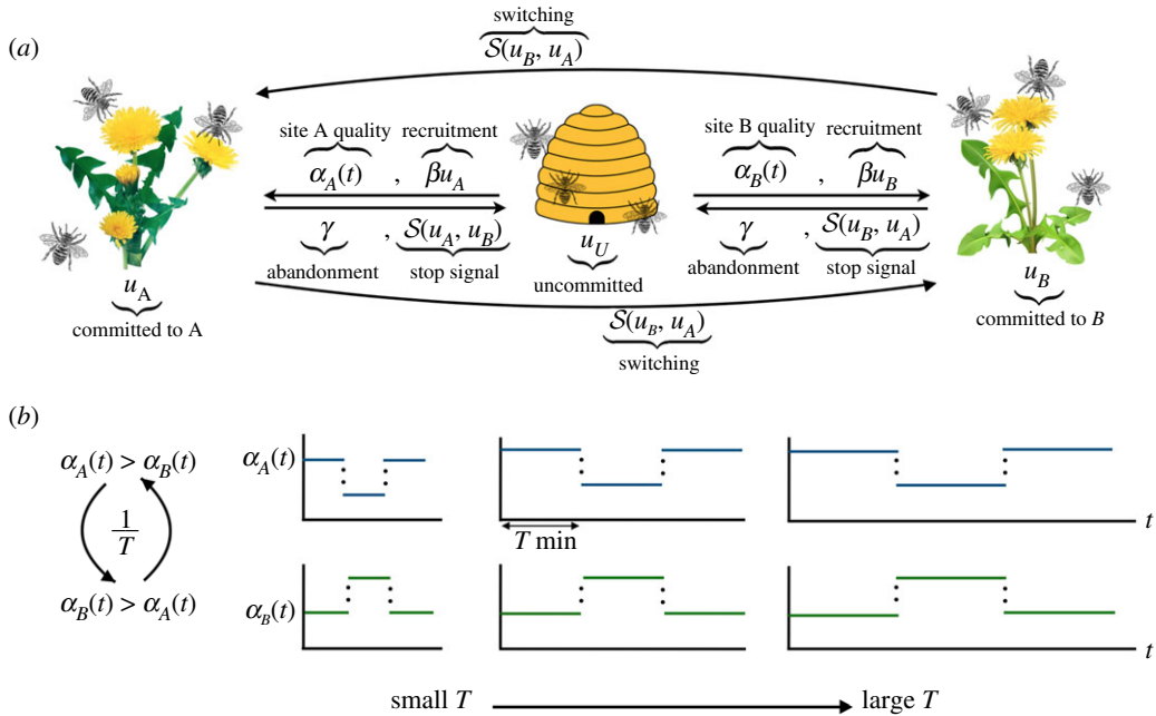
Figure 1. (a) Schematic of colony foraging model with two feeders (e.g. flowers or feeder boxes), equation (2.1). Bees move along arrows between different opinions (uncommitted or committed); arrow labels indicate interactions that provoke those opinion switches. (b) Example feeder quality time series \alpha_{A,B}(t) , which switch with period T min.
