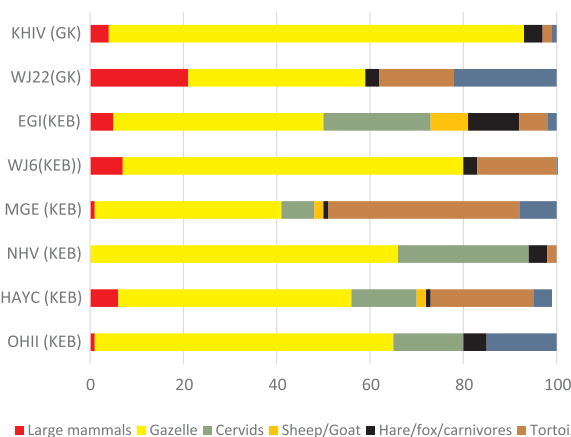
Fig. 4. Relative abundance (%) of prey at Kebaran (KEB) and Geometric Kebaran (GK) sites in the Levant. OHII = Ohalo II (Rabinovich and Nadel, 2005; Simmons and Nadel, 1998); HAYC = Hayonimc Cave C (Stiner, 2005); NHV = Nahal Hadera V (Bar-Oz 2004; Bar-Oz and Dayan 2002); MEG = Meged Rockshelter (Stiner 2005); WJ6 = Wadi Jilat 6 (Garrard and Byrd, 1992); EGI = Ein Gev I (Marom and Bar-Oz, 2008); WJ22 = Wadi Jilat 22 (Martin et al., 2013); KHIV = Kharaneh IV (present study).
