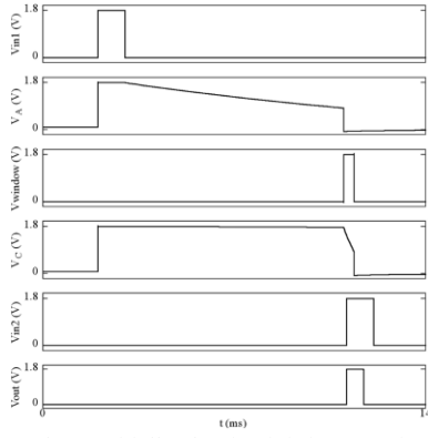
Fig. 4. Case 1: Na-Nb- \Delta t . Initially, the circuit is in non-coincidence mode ( V_{\text{coin}}=\text{gnd} ) and V_A and V_C are at logical 0. When a digital pulse arrives at V_{\text{in1}} , V_A and V_C rise as C1, C2, C3, and C4 charge up. When the pulse ends, V_A lowers as C1 and C2 begin to discharge at a rate determined by the user ( V_{\text{wstart}} ) and V_C lowers as C3 and C4 begin to discharge at a rate determined by the off current of NMOS M7 (very small). When V_A crosses \theta , it drops quickly to logical zero, V_{\text{window}} goes high, and V_C starts to lower more quickly as the discharge rate of C3 and C4 are now limited by V_{\text{winwidth}} (which is chosen by the user.) If a second digital pulse arrives at V_{\text{in2}} while V_{\text{window}} is high, V_{\text{patterndetected}} goes high and causes the pulse formatter circuit to generate a pulse on V_{\text{out}} and the refractory circuit to initiate a refractory period.
