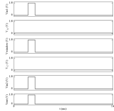
Fig. 6. Case 3: Na-Nb-coincidence. Initially, the circuit is in coincidence mode ( V_{\text{coin}}=V_{\text{dd}} ) and V_A and V_C are at logical 0. When a digital pulse arrives at V_{\text{in1}} , V_A and V_C remain unchanged as the output of U2 is held at logical 1 by V_{\text{coin}} . When a digital pulse arrives at V_{\text{in1}} , V_{\text{window}} goes high through U1 and U3. If a second digital pulse arrives at V_{\text{in2}} while V_{\text{window}} is high, V_{\text{patterndetected}} goes high and causes the pulse formatter circuit to generate a pulse on V_{\text{out}} and the refractory circuit to initiate a refractory period.
