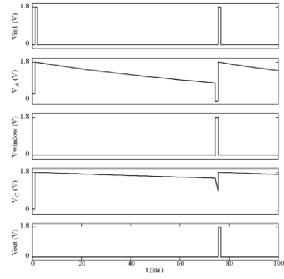
Fig. 5. Case 2: Na-Na- \Delta t . Initially, the circuit is in non-coincidence mode ( V_{\text{coin}}=\text{gnd} ), V_{\text{in1}} and V_{\text{in2}} are tied together, and V_A and V_C are at logical 0. When a digital pulse arrives at V_{\text{in1}} , V_A and V_C rise as C1, C2, C3, and C4 charge up. When the pulse ends, V_A lowers as C1 and C2 begin to discharge at a rate determined by the user ( V_{\text{wstart}} ) and V_C lowers as C3 and C4 begin to discharge at a rate determined by the off current of NMOS M7 (very small). When V_A crosses \theta , it drops quickly to logical zero, V_{\text{window}} goes high, and V_C starts to lower more quickly as the discharge rate of C3 and C4 are now limited by V_{\text{winwidth}} (which is chosen by the user.) If a second digital pulse arrives at V_{\text{in1}} while V_{\text{window}} is high, V_{\text{patterndetected}} goes high and causes the pulse formatter circuit to generate a pulse on V_{\text{out}} and the refractory circuit to initiate a refractory period. Also, V_A and V_C rise as C1, C2, C3, and C4 are recharged by the new pulse, cutting the window off and setting up the circuit to detect another Na-Na- \Delta t pattern.
