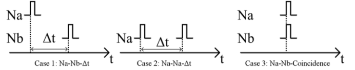
Fig. 1. The three fundamental spatiotemporal patterns that the circuit can detect. Case 1 illustrates the case where two outputs of two different neurons, Na and Nb, occur with some time, \Delta t , between them. Case 2 is a temporal pattern where a single neuron, Na, spikes twice with some time, \Delta t , between the spikes. Case 3 is a special case of Case 1 where \Delta t is reduced to zero so that the two spikes coincide.
