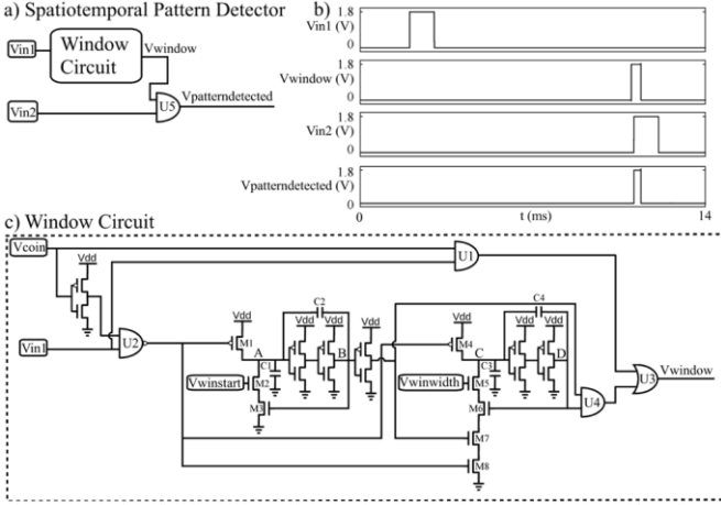
Fig. 2. a) A block diagram of the Spatiotemporal Pattern Detector. b) The response of the spatiotemporal pattern detector to stimulus with Vcoin tied to gnd. The pulses applied to Vin1 and Vin2 are 1.8 V for duration 1 ms. c) Schematic of the window circuit.
