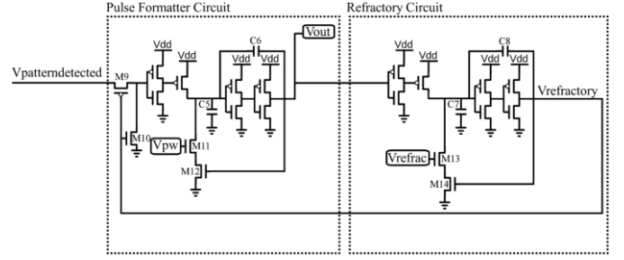
Fig. 3. The Pulse Formatter and Refractory circuits. The pulse Formatter takes Vpatterndetected signals and produces an output pulse of a width determined by the user set Vpw. The Refractory circuit produces a signal, Vrefractory, which prevents Vpatterndetected signals from reaching the Pulse Formatter Circuit.
