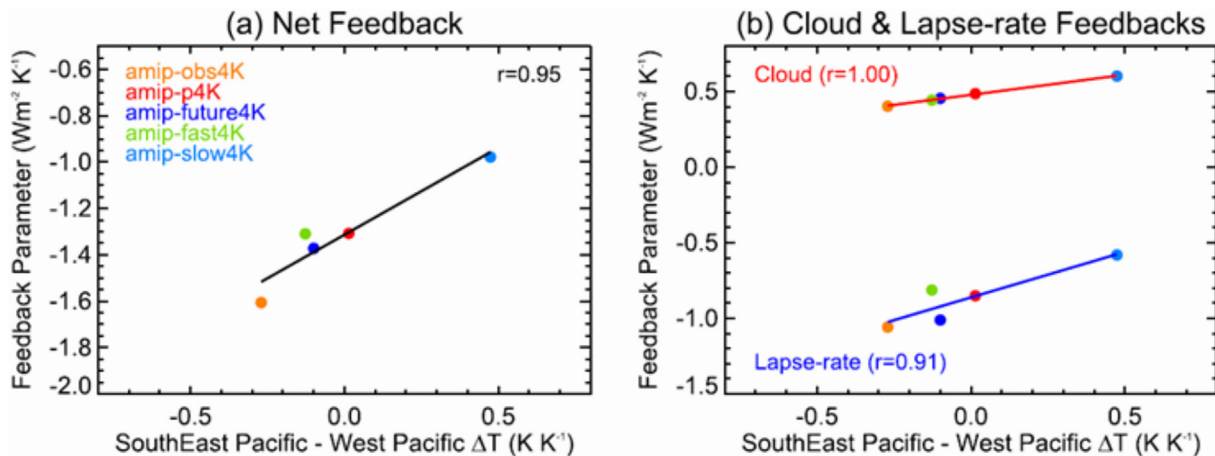
Fig. 3. Dependence of (a) net and (b) cloud and lapse-rate feedbacks on sea surface warming patterns. Feedbacks are determined through simulations of the Hadley Centre Global Environmental Model, version 2 and compared against control simulations forced with monthly observed SST and all forcing agents from 1979 to 2008. The perturbation experiments are the same as the control simulation but with perturbed SST forcing scaled to ensure a global-mean SST increase of 4 K and a warming pattern determined by: observed 20th century trends (amip-obs4K), uniform warming of 4 K (amip-p4K), CGCMs forced by a 1% yr -1 CO 2 increase (amip-future4K), years 1–20 (amip-fast4K) and years 21–150 (amip-slow4K) from CGCMs forced by an abrupt quadrupling of CO 2 . The warming pattern (x-axis of each panel) is defined as the temperature change difference between the southeast tropical Pacific (30°S–0°, 260°–280°E) and the west Pacific (15°S–15°N, 150°–170°E). Figure from Andrews and Webb (2018). © Copyright 15 January 2018 American Meteorological Society (AMS).
