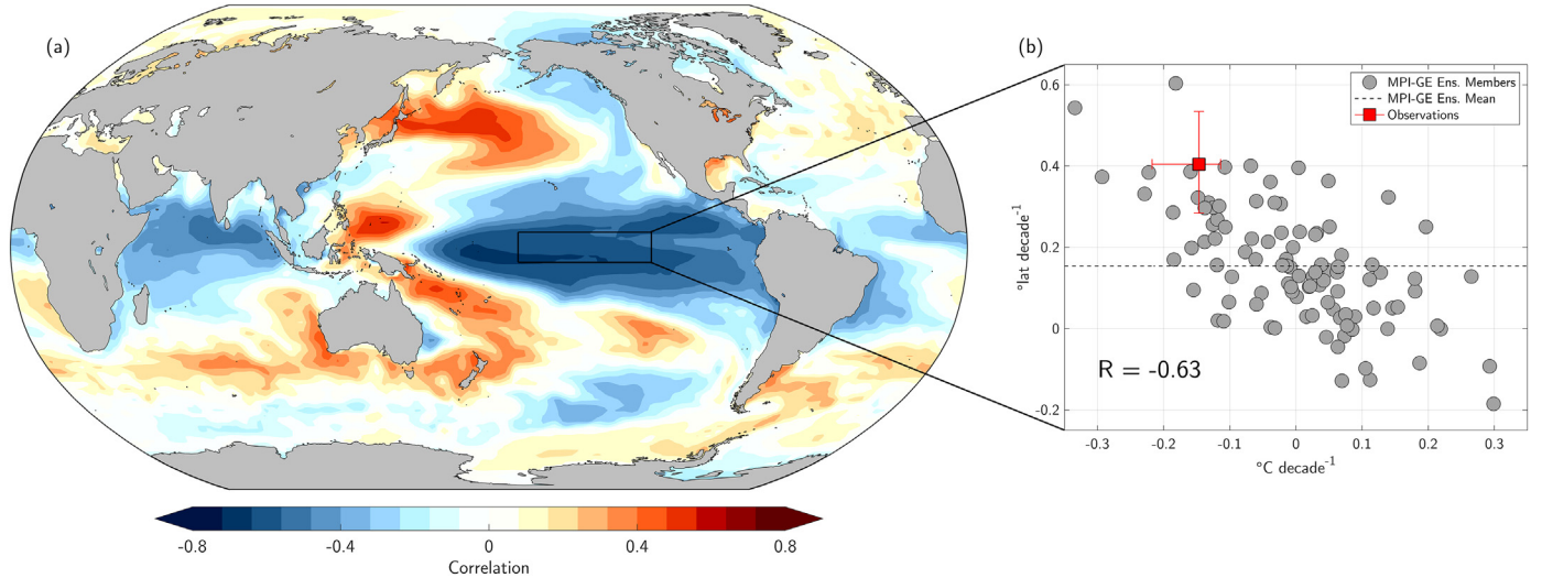
Fig. 9. Relationship between Hadley cell expansion/contraction and Pacific sea surface temperatures. (a) Correlation (shading) of 100 total (NH + SH) \psi_{500} = 0 trends with 100 SSTA* trends at each grid point using MPI-GE from 1985 to 2014. (b) Scatter plot of total \psi_{500} = 0 trends (y-axis; ^{\circ}\text{lat decade}^{-1} ) and SSTA trends averaged in the Niño3.4 region (x-axis; ^{\circ}\text{C decade}^{-1} ). Grey circles represent trends derived from MPI-GE. Dashed black line indicates MPI-GE total \psi_{500} = 0 ensemble mean. Note that MPI-GE Niño3.4 trends are relative to the ensemble mean (i.e., Niño3.4*). Red box and whiskers represent the median and range, respectively, of trends derived from observed products. Observed total \psi_{500} = 0 trends calculated using ERA-Interim, ERA5, MERRA2 (analyzed), and JRA-55. Observed Niño3.4 trends calculated using ERSSTv3b, ERSSTv5, HadISSTv1.1, and ICOADS.
