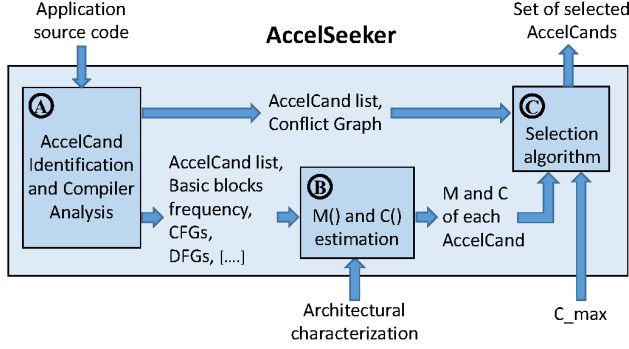
Fig. 2. The phases of the AccelSeeker approach. A) Candidates for acceleration are identified, from source code analysis. B) Given an estimation of merit and cost for each candidate, and C) given a maximum available cost, AccelSeeker performs selection of a subset of such candidates.
