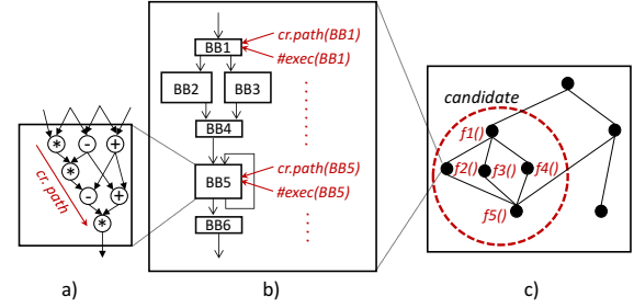
Fig. 6. Estimation of hardware computation times at the basic block (a), function (b) and AccelCand (c) levels.
