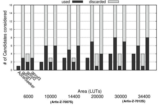
Fig. 10. Number of candidates selected by AccelSeeker and, for comparison, by the gprof -based strategies, while varying the area constraints. Candidate accelerators selected by gprof exceeding resource constraints can only be discarded after their implementation.
