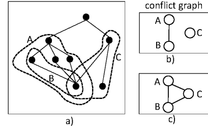
Fig. 4. a) Three overlapping AccelCands: A, B, C. b) Conflict graph considered in our problem formulation: complete overlap is a conflict, while partial overlap is allowed. c) Conflict graph adopted in [25] instead, where any kind of overlap is considered a conflict.
