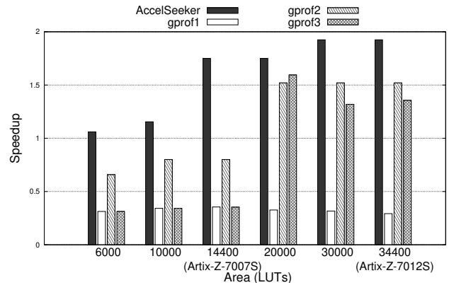
Fig. 8. Speedup obtained over the whole runtime of H.264 decoder by implementing, as hardware accelerators, the candidate sets obtained with AccelSeeker and the ones retrieved by gprof1 , gprof2 and gprof3 profiling strategies (as detailed in VII-B), varying the area constraint.
