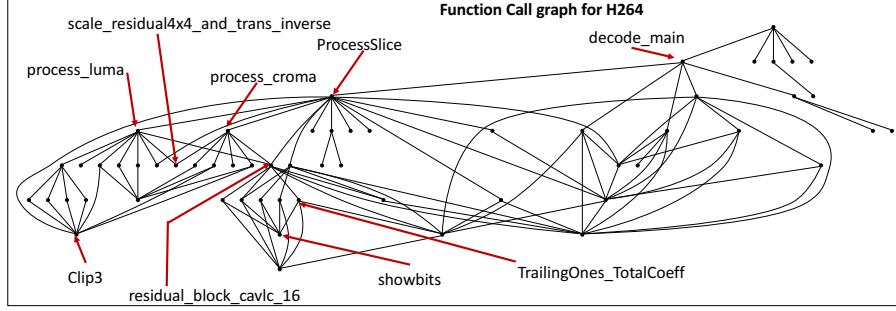
Fig. 7. Call graph of H.264, with some function names highlighted.
