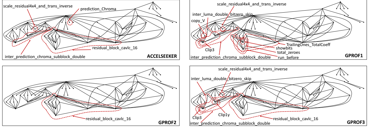
Fig. 9. H.264 call-graphs highlighting the acceleration candidates selected by by AccelSeeker, and by the three gprof strategies, for a 30k LUTs area budget.
