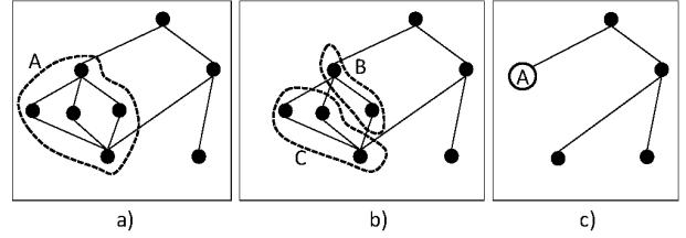
Fig. 3. a) An example call graph. Black nodes are the functions present in a SW application, and edges represent function calls. Subgraph A is an AccelCand. b) Subgraphs B and C are not AccelCands (B has outgoing edges, C has no root). c) Call graph resulting from selection of A as accelerator.
