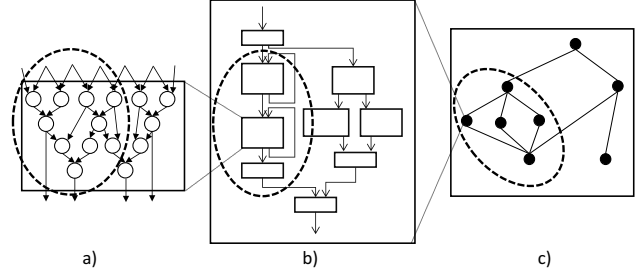
Fig. 1. Evolution of the SoA in automatic selection of custom instructions/accelerators: (a) from data-flow level [23] [24], (b) to control-flow level [25] [26], (c) to function-call graph level (this work).
