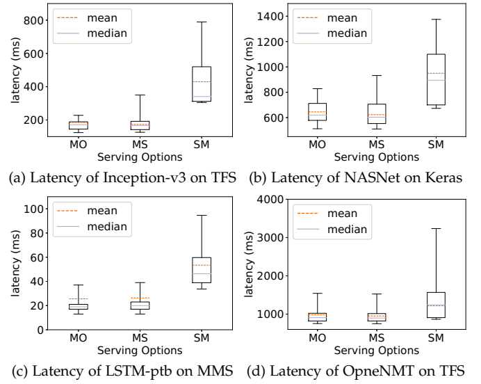
Fig. 7: Latency comparison of MARK-ondemand (MO), MARK-spot (MS), and SageMaker (SM) on 4 ML models using Twitter workload.
