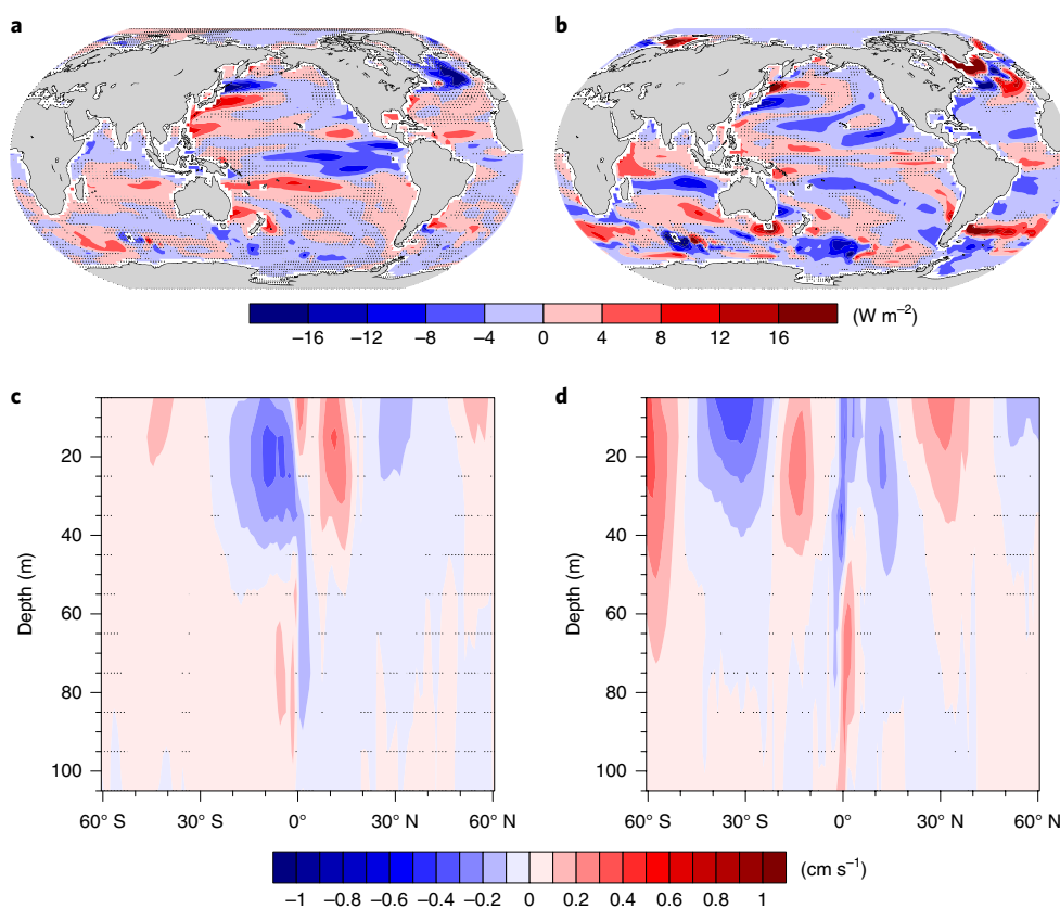
Fig. 3 | Ocean response to CO 2 forcing. a–d. Ensemble-mean net surface heat flux from the ocean to the atmosphere for EQ CPL (a) and OFFEQ CPL (b), as well as ensemble-mean zonal-mean meridional ocean currents for EQ CPL (c) and OFFEQ CPL (d). Values that are not significantly different from zero at the 95% confidence level are indicated by black stippling (using a local two-tailed t -test) and additional grey stippling (using FDR-adjusted critical P values).
