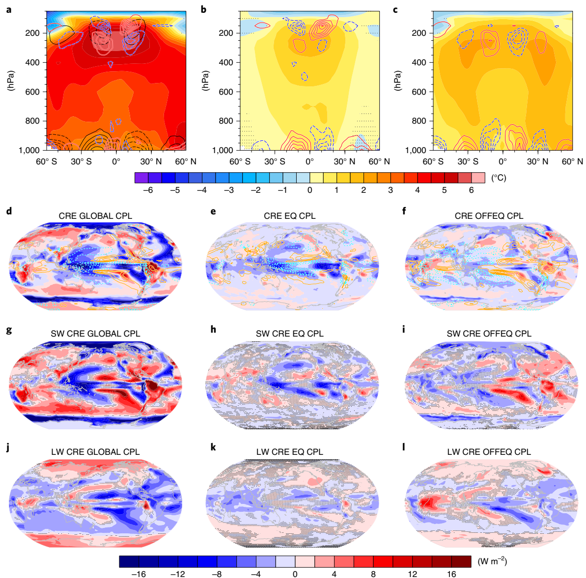
Fig. 2 | Ensemble-mean temperature, meridional wind, vertical pressure velocity and cloud radiative effect (CRE) responses to \text{CO}_2 forcing. a–c , Zonal-mean temperature (shading) and meridional wind (coloured contours; solid red indicating positive values and dashed blue negative values) responses for GLOBAL CPL (interval: 0.1 \text{ m s}^{-1} ) ( a ), EQ CPL (interval: 0.05 \text{ m s}^{-1} ) ( b ) and OFFEQ CPL (interval: 0.05 \text{ m s}^{-1} ) ( c ). The climatological zonal-mean meridional wind is overlaid in black contours (interval: 0.5 \text{ m s}^{-1} ) in a to indicate the climatological Hadley circulation inflow and outflow. d–f , Total CRE ( d–f ) and LW CRE ( j–l ) for GLOBAL CPL ( d,g,j ), EQ CPL ( e,h,k ) and OFFEQ CPL ( f,i,l ). The vertical pressure velocity response at 500 hPa is overlaid in coloured (solid orange for positive values and dashed cyan for negative values) contours (intervals: 0.006 \text{ Pa s}^{-1} for GLOBAL and 0.003 \text{ Pa s}^{-1} for EQ and OFFEQ) in d–f . Ensemble-mean temperature, SW CRE and LW CRE values that are not significantly different from zero at the 95% confidence level are indicated by black stippling (using a local two-tailed t -test) and additional grey stippling (using FDR-adjusted critical P values) in a–c and g–l . Zero contour lines are omitted.
