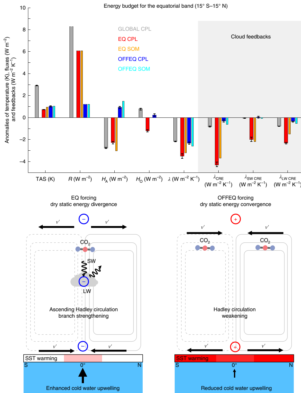
Fig. 4 | Feedback mechanism. Top, Anomalies of TAS, effective radiative forcing ( R ), net heat flux from the ocean to the atmosphere ( H_O ), heat convergence due to atmospheric heat transport ( H_A ), the total feedback parameter ( \lambda ), as well as the total ( \lambda_{\text{CRE}} ), SW ( \lambda_{\text{SW CRE}} ) and LW ( \lambda_{\text{LW CRE}} ) cloud feedbacks for the equatorial band. Error bars indicate the ensemble range of the responses and the calculated feedback for the coupled experiments. Bottom, Schematic summary of the physical processes explaining the differing surface temperature response to EQ (left) and OFFEQ (right) forcing where v' is the anomalous zonal-mean meridional wind in the upper and lower troposphere.
