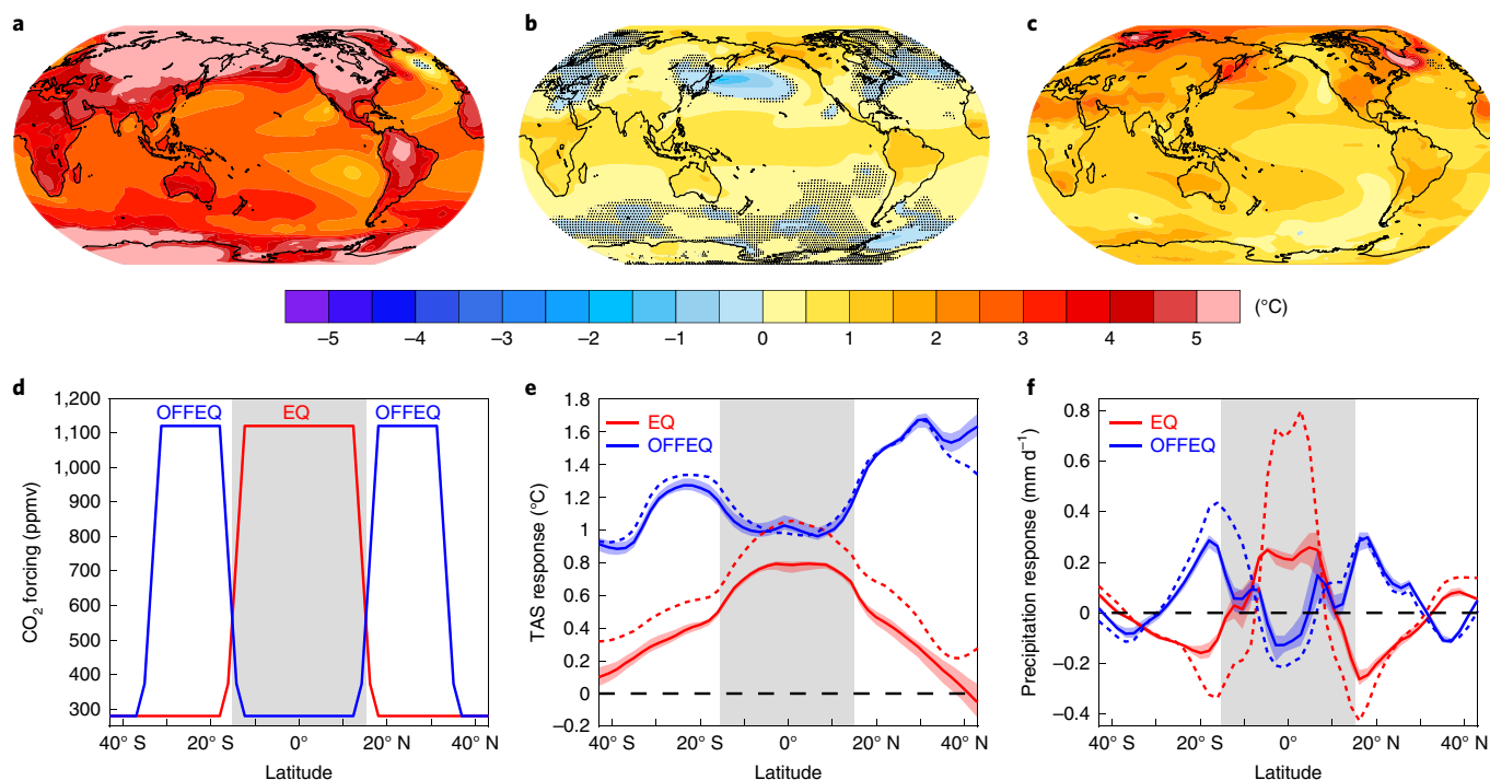
Fig. 1 | Surface temperature and precipitation response to CO 2 forcing. a–c , TAS response for GLOBAL CPL ( a ), EQ CPL ( b ) and OFFEQ CPL ( c ). Values that are not significantly different from zero at the 95% confidence level are indicated by black stippling (using a local two-tailed t -test) and additional grey stippling (using FDR-adjusted critical P values). d , CO 2 forcing for the EQ and OFFEQ regional forcing experiments. e , Zonal-mean TAS response for EQ CPL (solid red), OFFEQ CPL (solid blue), EQ SOM (dashed red) and OFFEQ SOM (dashed blue). f , Zonal-mean precipitation (P) response for the same experiments as in e . Red and blue shading in e and f indicates the ensemble range of the responses. Grey shading in d–f indicates the equatorial region.
