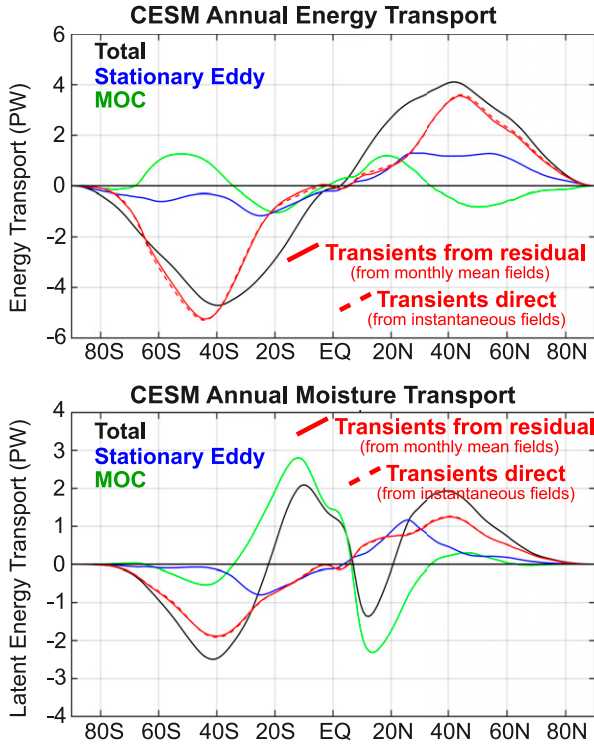
FIG. 3. Comparison of the zonally and vertically integrated transient eddy energy transport in CESM calculated using the residual method (section 2b; solid red lines) and the direct method (section 2a; dashed red lines). (top) The total annual-mean atmospheric energy transport. (bottom) The annual-mean atmospheric moisture transport.
