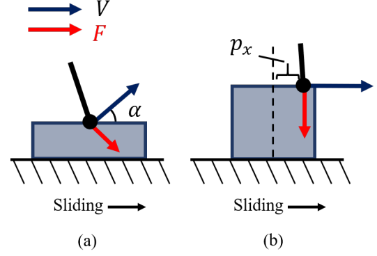
Fig. 7. The two test settings. In test one, we change the angle \alpha of velocity control. In test two, we change the location p_x of the contact point.
