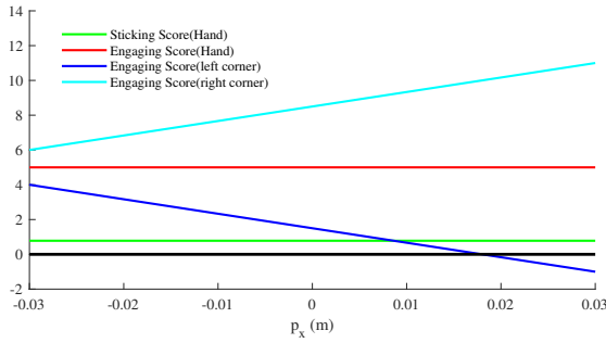
Fig. 9. The force-related robustness scores in test setting two.
