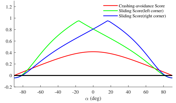
Fig. 8. The velocity-related robustness scores in test setting one.
