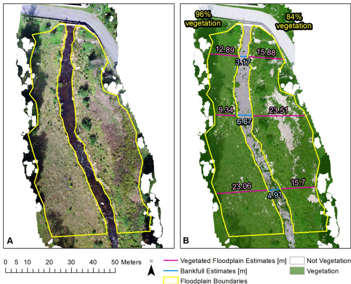
Figure 8: An example of how remote sensing and GIS can be used to calculate “true” ecological evaluation metrics analogous to the SVAP2 metrics. Specifically, this example depicts how this approach can calculate metrics related to the riparian area quantity element in the SVAP2. (A) MA site orthomosaic with assessment area. (B) MA site orthomosaic with partially transparent binary raster overlay showing the vegetation coverage throughout the site. A binary raster of vegetation cover was created in ArcGIS by using the raster calculator to first calculate the Green Leaf Index (GLI; Louhaichi et al. 2001), then again to select pixels with GLI values greater than
