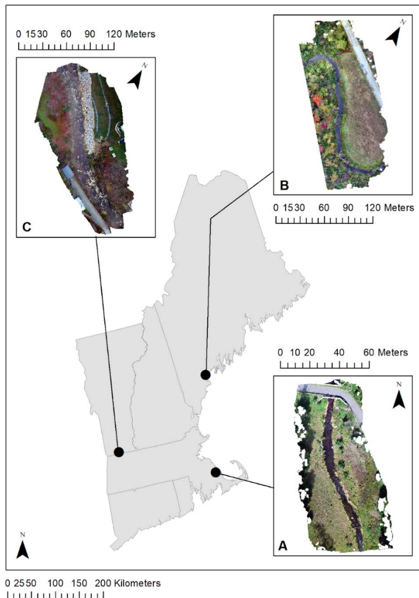
Figure 1: The three sites selected from the stream reaches visited by the USACE during their SVAP2 tour. (A) Town Brook in Plymouth, MA. (B) East Branch Piscataqua River in Falmouth,
