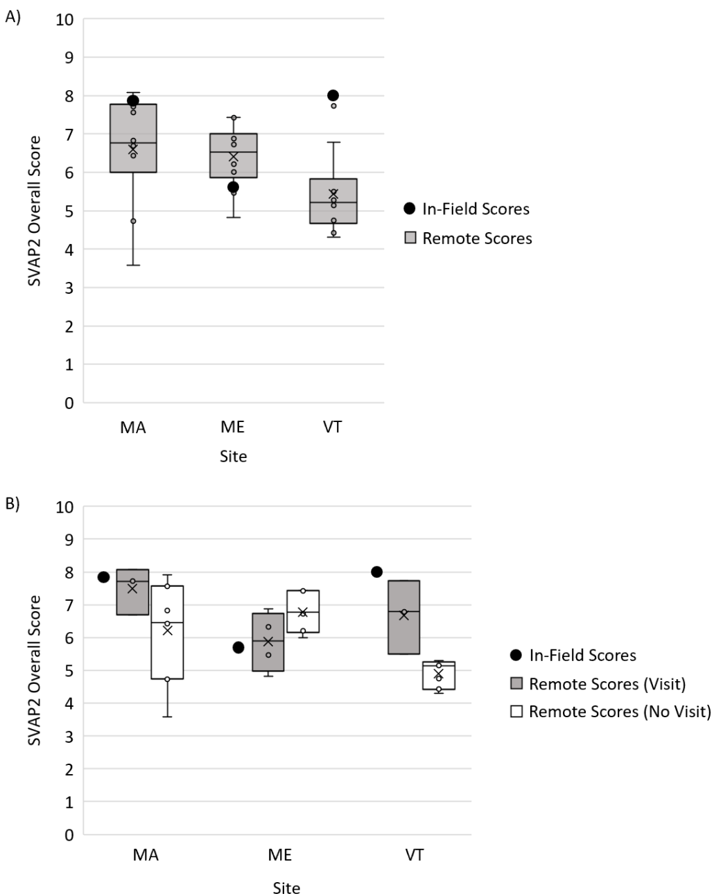
Figure 6: A comparison the remote overall SVAP2 scores provided by each survey participant to the score determined by the USACE team out in the field. “X” markers in box plots represent the
