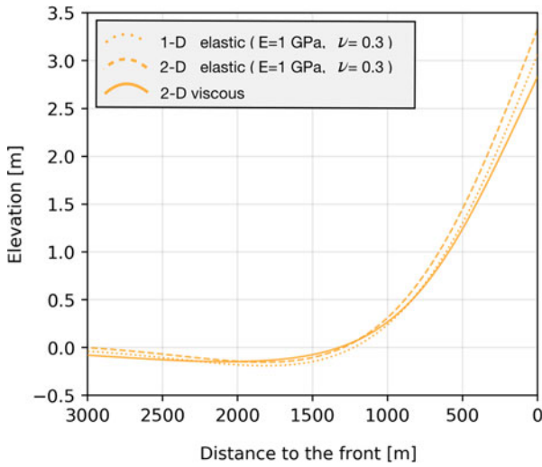
Fig. 7. Example of elastic and early-stage viscous ( t = 0.005 \text{ a} ) rampart-moat for E = 1 \text{ GPa} , \nu = 0.3 and l_{\text{foot}} = 50 m.
