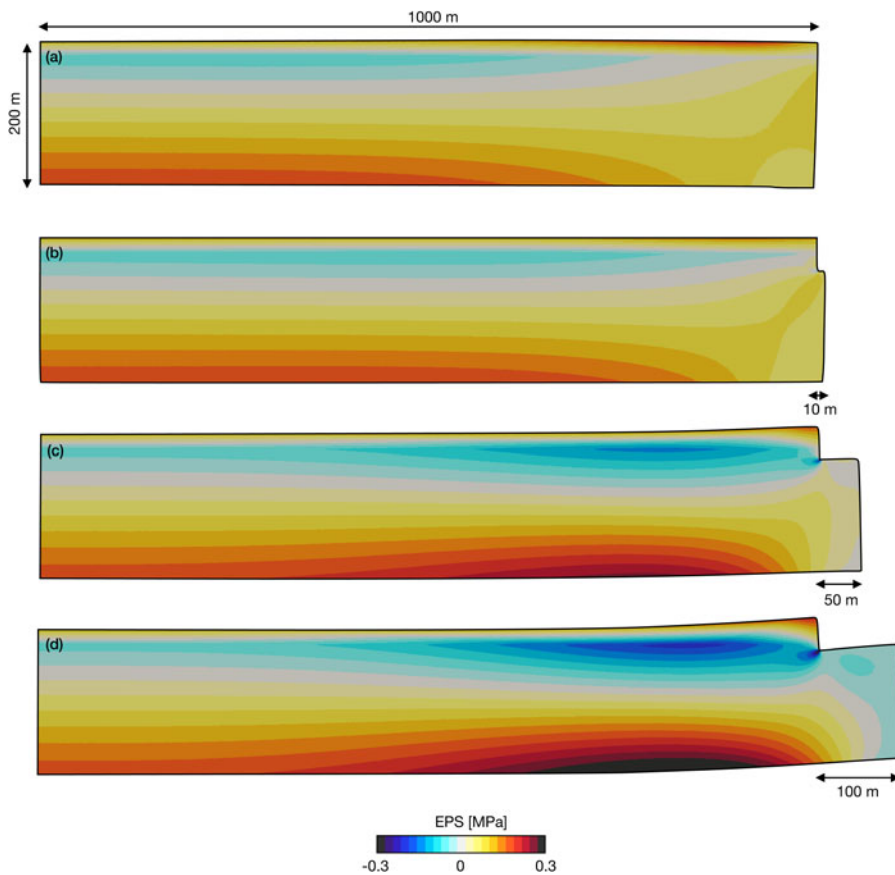
Fig. 8. Elastic (for E_{2-D} = 10 MPa and \nu = 0.3 ) effective principal stress for an underwater foot of length (a) 0 m, (b) 10 m, (c) 50 m and (d) 100 m. These elastic solutions exhibit the full deformation produced by the buoyancy stress. Only the portion of the ice shelf within 1000 m of the front is shown.
