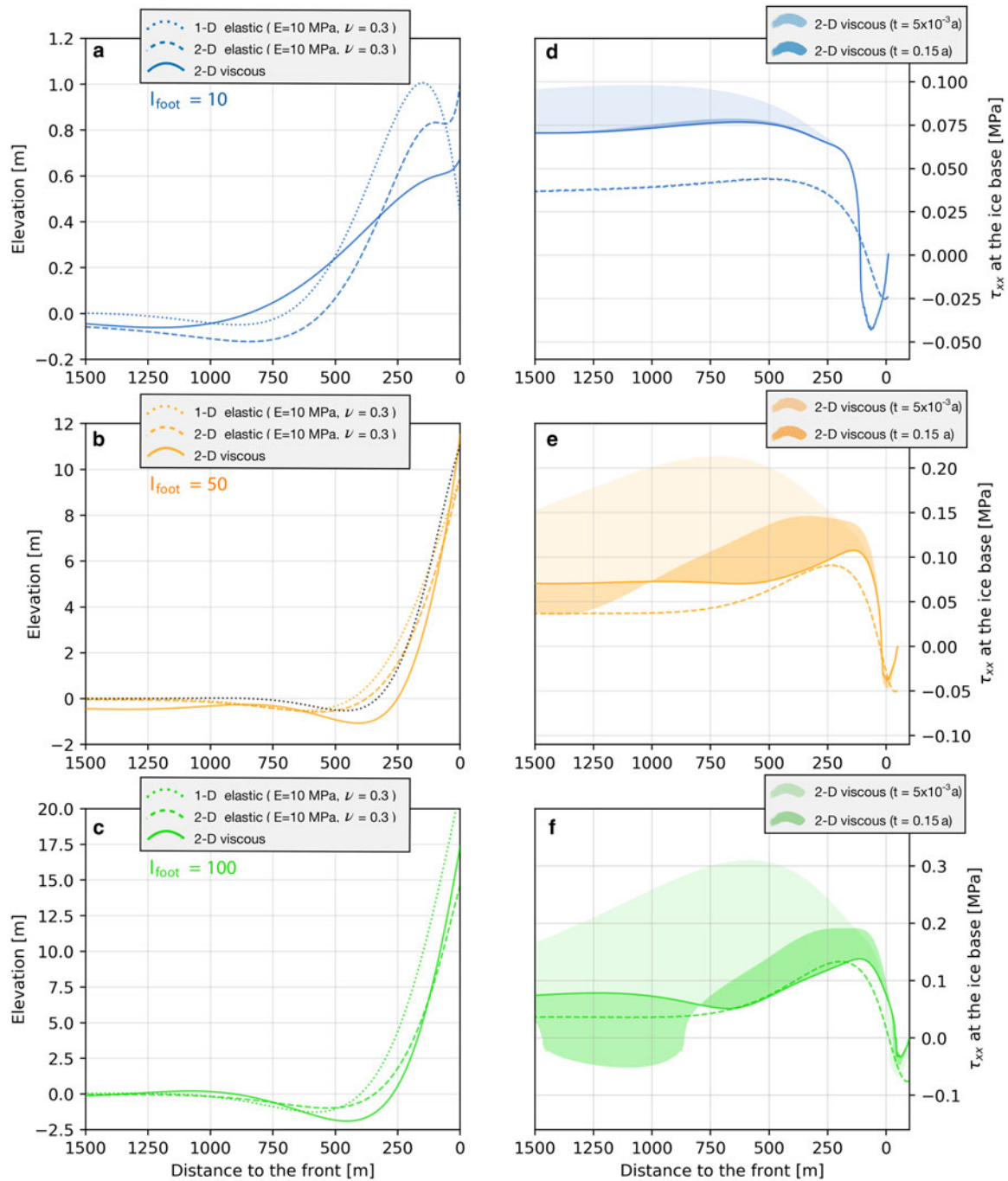
Fig. 5. Left: rampart-moat geometry predicted by viscous and elastic ( E = 10 MPa and \nu = 0.3 ) models, for various lengths of underwater foot for the 1500 m closest to the ice front: (a) l_{\text{foot}} = 10 m; (b) l_{\text{foot}} = 50 m; and (c) l_{\text{foot}} = 100 m. The 1-D analytical elastic rampart-moat solution for the parameters E = 2 MPa and l_{\text{foot}} = 40 m, discussed in Section 4.2, is plotted in black in panel (b). Right: longitudinal deviatoric stress at the ice base for the viscous and 2-D elastic frameworks, for each value of l_{\text{foot}} . The shading represents the envelope of the stresses for the viscous framework from the beginning of the simulation (light shades) and from 0.15 a (dark shades) to the final stress (continuous lines). The 2-D elastic stresses are shown as dashed lines.
