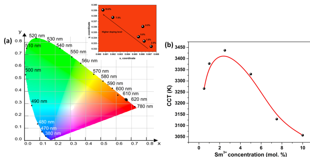
Figure 3. (a) CIE index diagram (excited at 405 nm) and (b) variation of the CCT with Sm 3+ doping concentration of the LHOs NPs. The inset of Figure 3a shows the magnified color coordinates of the LHOs NPs with different Sm 3+ concentrations.
