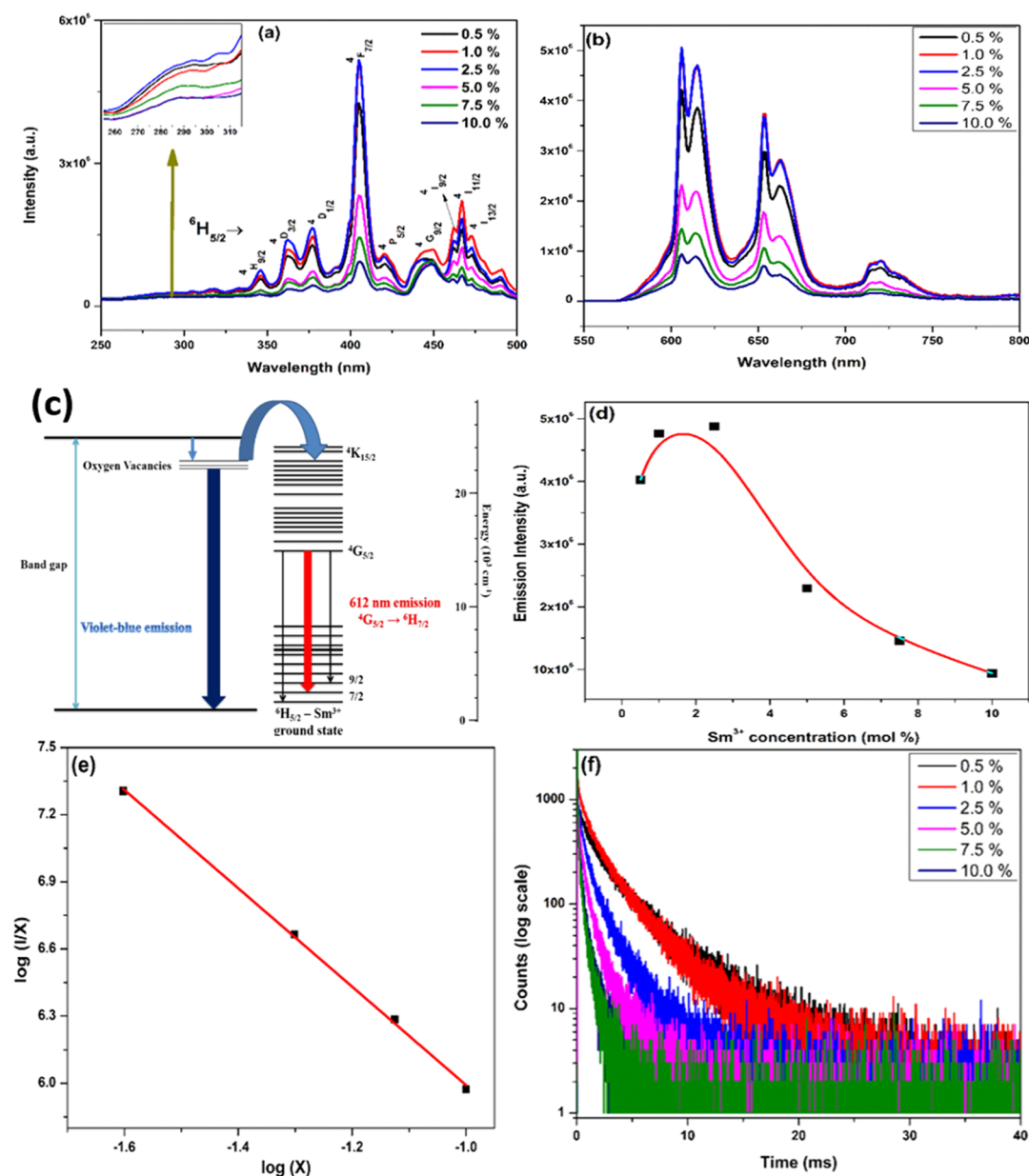
Figure 2. (a) PL excitation spectra ( \lambda_{\text{em}} = 607 nm), (b) PL emission spectra ( \lambda_{\text{ex}} = 405 nm), (c) proposed mechanism of host-to-dopant energy transfer, (d) variation of integrated emission intensity in the range of 575–675 nm as a function of Sm 3+ doping concentration, (e) relation between \log_{10}(I/x) and \log_{10}(x) based on the Van Uitert equation, and (f) luminescence decay profiles of the LHOS NPs with Sm 3+ doping level from 0.5 to 10.0%. The inset of Figure 1a shows the magnified excitation spectra in the wavelength range of 260–315 nm.
