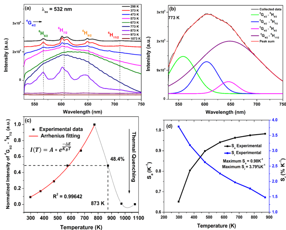
Figure 5. LHOS (2.5%) NPs: (a) in situ PL spectra measured from 298 to 1073 K. (b) Deconvoluted electronic transition peaks of \text{Sm}^{3+} ions at 773 K. (c) Arrhenius plot of the integrated PL intensity of ^4G_{5/2} \rightarrow ^6H_{7/2} transition from 298 to 1073 K. (d) Variation of S_a and S_r as a function of temperature.
