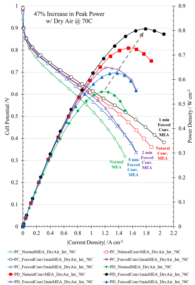
Fig. 7 H 2 -Air PEMFC discharge polarization and power density curves for normal MEA, natural convection MEA, and forced convection MEAs with different purge times at 70 °C using humidified hydrogen and dry air
