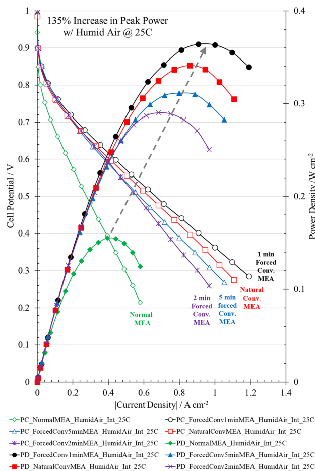
Fig. 5 H 2 -Air PEMFC discharge polarization and power density curves for normal, natural and forced convection MEAs with different purge times at 25 °C using humidified hydrogen and humidified air
