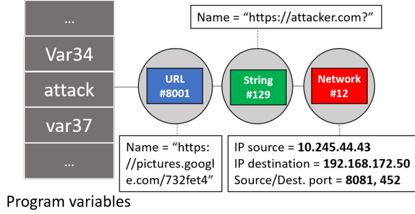
Fig. 2. Provenance list of the variable attack (related to url Upload Attack.)
