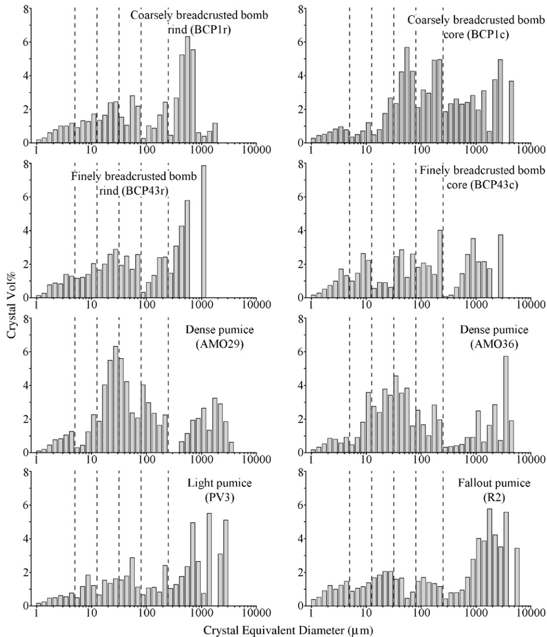
Fig. 13. Glass-referenced crystal volume distributions.
