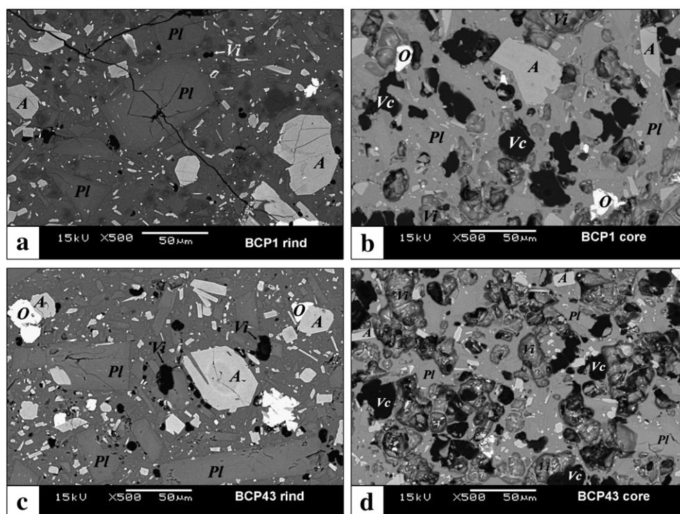
Fig. 9. Backscattered SEM images of breadcrust bombs. All the images are at the same scale. Labels are: (A) amphibole, (Pl) plagioclase, (O) oxide, (Vc) connected vesicle, (Vi) isolated vesicle. a) Coarsely breadcrusted bomb rind containing rare small isolated vesicles. Note that the bomb rinds are typically very heterogeneous, and vesicles are not present everywhere. The occurrence of areas of rind free of vesicles shows that the coarsely breadcrusted bombs inflated from essentially non-vesicular magma. b) Vesicular interior of coarsely breadcrusted bomb core containing both isolated (non-impregnated; grey) and connected (impregnated; black) vesicles. c) Finely breadcrusted bomb rind with patchily distributed small vesicles; note the higher vesicle numbers than in the rind of the coarsely breadcrusted bomb (a). d) Finely breadcrusted bomb core containing the same two types of vesicles as the coarsely breadcrusted bomb (b), but in greater abundance.
