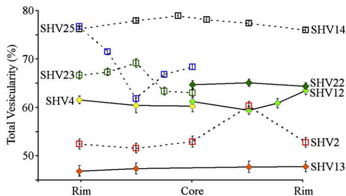
Fig. 4. Vesicularity as a function of relative position inside large pumices (>30 cm). Filled diamonds with solid lines are those pumices that were judged in the field to be texturally homogeneous; squares with dashed lines are those that had larger vesicles in the interior than in the rind.
