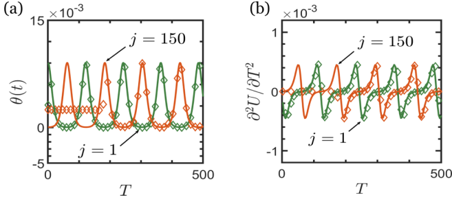
FIG. 3. Comparison between the numerical results (diamonds) obtained by solving the 2N discrete differential equations [Eq. (1)] and the analytical (solid lines) results [Eqs. (4) and (9)]: (a) \theta and (b) \partial^2 U / \partial T^2 for f = 25 Hz and \kappa^2 = 0.90 .
