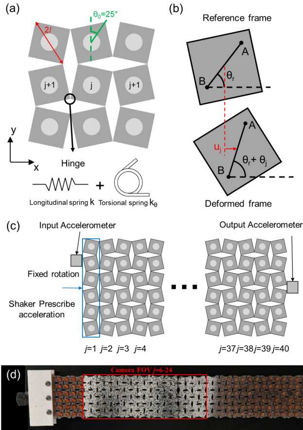
FIG. 1. (a) Schematic of the system and geometry of the squares. (b) Displacement and rotation of each square. (c) Experimental setup including a shaker that provides the cnoidal wave input and accelerometers at both ends that measure the input and output acceleration. (d) Image of the entire sample, with the portion recorded via a high-speed camera indicated by the red rectangle.
