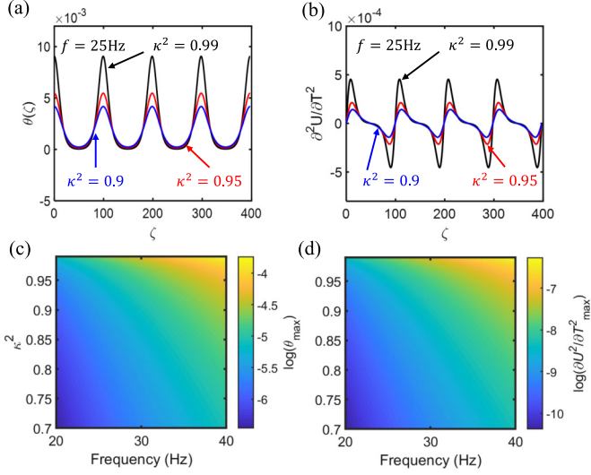
FIG. 2. Analytical cnoidal wave solutions for f = 25 Hz and \kappa^2 = 0.99, 0.95 , and 0.90 : (a) \theta(\zeta) = A \text{cn}^2(\frac{\zeta}{W}|\kappa^2) + B [Eq. (4)]; (b) \partial^2 U / \partial T^2(\zeta) [Eq. (9)]; (c, d) amplitude of \theta and \partial^2 U / \partial T^2 solution vs f and \kappa^2 .
