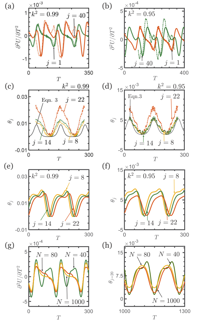
FIG. 4. The comparison between experimental (dash lines) and numerical results (solid lines) of \partial^2 U / \partial T^2 data for f = 25 Hz and \kappa^2 = (a) 0.99 and (b) 0.95. Experimental result of \theta (dash lines) compared to analytical solution (solid line) for f = 25 Hz and \kappa^2 = (c) 0.99 and (d) 0.95. Numerical result of \theta for f = 25 Hz and \kappa^2 = (e) 0.99 and (f) 0.95. Numerical result of systems with various sample length ( N ) for \kappa^2 = 0.95 : (g) \partial^2 U / \partial T^2 and (h) \theta_{j=20} .
