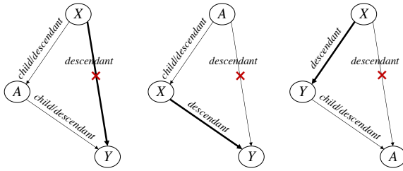
Figure 5: Remove redundancy when adding \text{ancestor}(X, Y) to the hierarchy.
