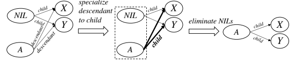
Figure 6: Two scenarios that NIL nodes can be eliminated when finalizing the hierarchy.
