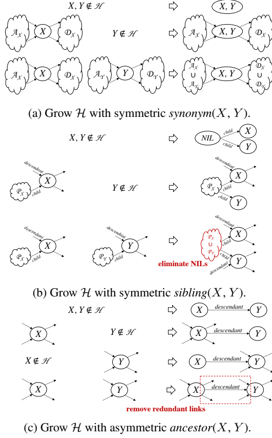
Figure 4: Hierarchy growth with a new relation.
