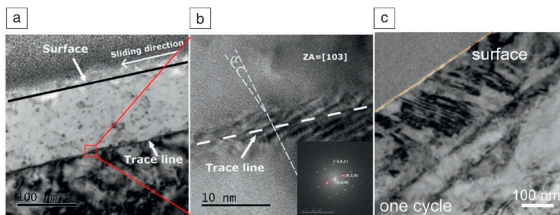
Figure 7. Dislocation self-organization during the very early stages of sliding leads to a horizontal small-angle grain-boundary-like feature, which can be observed using transmission electron microscopy after only a single sliding event (a, b). The foil was tilted to a [103] zone axis (ZA). 93 The line-like feature was found to be a boundary separating regions that accommodate shear differently, with dislocation motion dominant below the line and twinning dominant above, as shown in (c). 95
