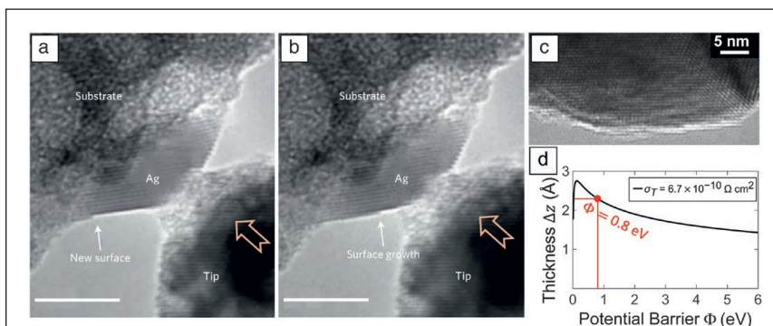
Figure 6. In situ transmission electron microscopy compression of silver contacts shows 80 that deformation is accommodated through the motion of surface steps (a, b). Scale bars = 5 nm. However, subsurface defect-based plasticity is observed 85 in platinum nanocontacts (c), and real-time electrical measurements 86 are consistent with the presence of atomic-scale surface layers (d), which may disrupt surface diffusion. (a, b) Reprinted with permission from Reference 80. © 2014 Nature Publishing Group. (c, d) Reprinted with permission from Reference 86. © 2019 IOP Publishing.
