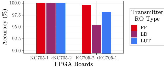
Fig. 19: The accuracy between the two Kintex 7 boards is consistently high for all types of source ROs tested.
