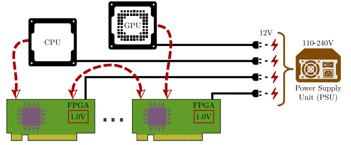
Fig. 1: System model for FPGA-to-FPGA, CPU-to-FPGA, and GPU-to-FPGA leakage in co-located environments. The CPU, GPU, and one or more (potentially malicious) FPGAs are powered through the same PSU, but do not share any logic, and do not have access to system monitors for measuring voltage or temperature changes.
