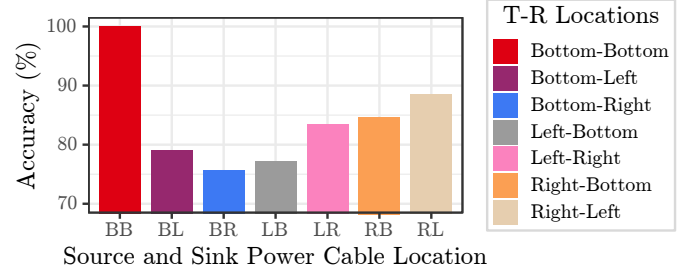
Fig. 18: Accuracy of communication between the two Kintex 7 boards in different cable arrangements.
