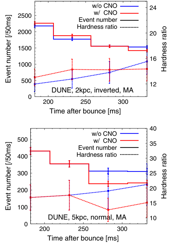
FIG. 17. Same as Fig. 12 but for the FD initial spectra.
