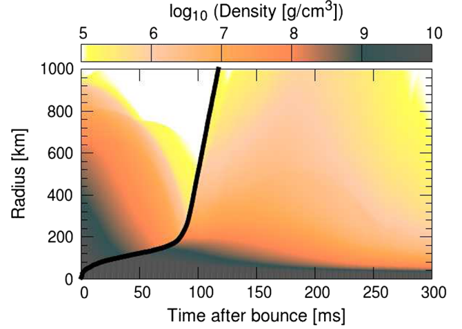
FIG. 1. The black curve is the time evolution of the shock radius. The colored areas show the time evolution of the logarithmic density profile [\text{g}/\text{cm}^3] . The horizontal axis is the time after bounce in ms, and the vertical axis shows the radial coordinates in km.
