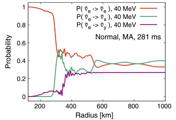
FIG. 8. The radial profiles of conversion probabilities of electron antineutrinos at 281 ms postbounce in the normal mass hierarchy. The different colors show the profiles of different conversion probabilities of \bar{\nu}_e : P_{e\alpha} = P(\bar{\nu}_e \rightarrow \bar{\nu}_\alpha) ( \alpha = e, x, y ) whose energy is 40 MeV. The red, green, and violet lines correspond to P_{ee} , P_{ex} , and P_{ey} , respectively.
