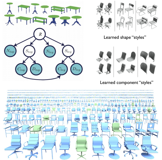
Figure 13: Top left : A Bayesian network [KCKK12] trained on a toy table dataset with two part labels. R and S are latent variables that mediate correlations between observed features (blue circles). Top right : A full network trained on segmented and labeled chairs learns to associate stylistic clusters with different latent variable values. Bottom : Novel chairs (blue) sampled from a model trained on 88 chairs (green). Note that stylistic constraints are preserved.
