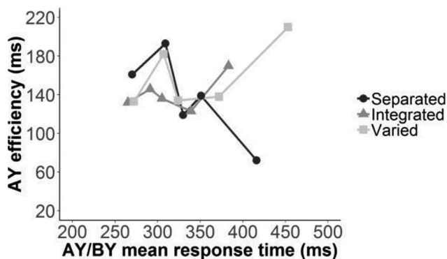
Figure 6. Delta plots showing the condition difference as a function of quintile scores across bilinguals in each context. Delta plots show an effect size (i.e., the difference between AY and BY response times [RTs]) as a function of response speed across participants (i.e., the average AY and BY RT for any given participant). This is achieved by ordering and dividing RTs for each participant into quintiles. More positive values on the y-axis indicate slower AY responses relative to BY trials. More positive values on the x-axis indicate individuals with slower RTs across the two conditions. Response inhibition is typically assumed to require time to unfold (De Jong, Liang, & Lauber, 1994; Ridderinkhof, Scheres, Oosterlaan, & Sergeant, 2005; Ridderinkhof, Van den Wildenberg, Wijnen, & Burle, 2004). In this case, reduced interference effects (i.e., high AY efficiency) should emerge for individuals with slower overall responses. This pattern is observed for bilinguals in the separated context, which is also consistent with the pattern reported by Morales and colleagues (2013), who also tested Spanish–English bilinguals from the same community in Spain. On the other hand, bilinguals in integrated and varied contexts showed the opposite trend (i.e., high AY efficiency emerged for individuals with faster overall responses), suggesting that, for these individuals, high AY efficiency is achieved via context monitoring procedures. A and B represent cues; X and Y represent probes.
