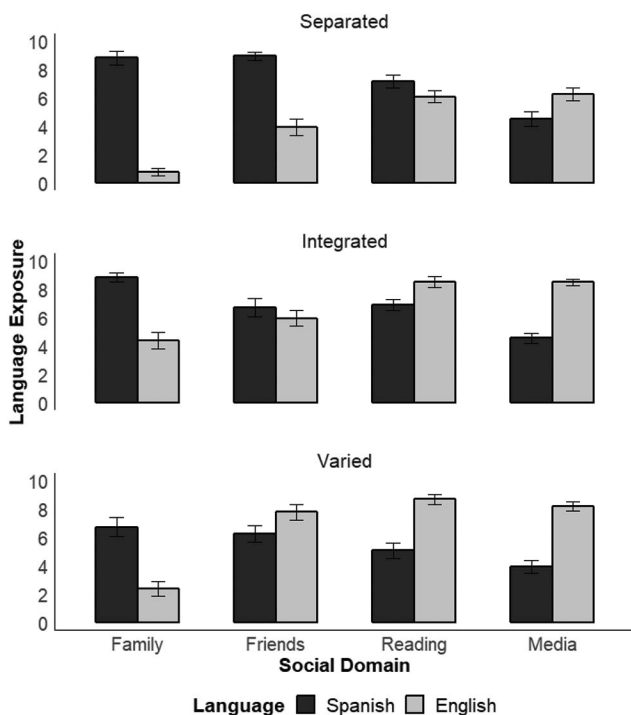
Figure 1. Participants' self-reported exposure to Spanish and English across different social domains. Ratings were made on a 10-point scale ranging from 0 ( no exposure ) to 10 ( high exposure ). Error bars indicate standard error of the mean. See Table S2 in the online supplemental materials for mean values, standard deviations, confidence intervals, and valid N for each measure per group.
