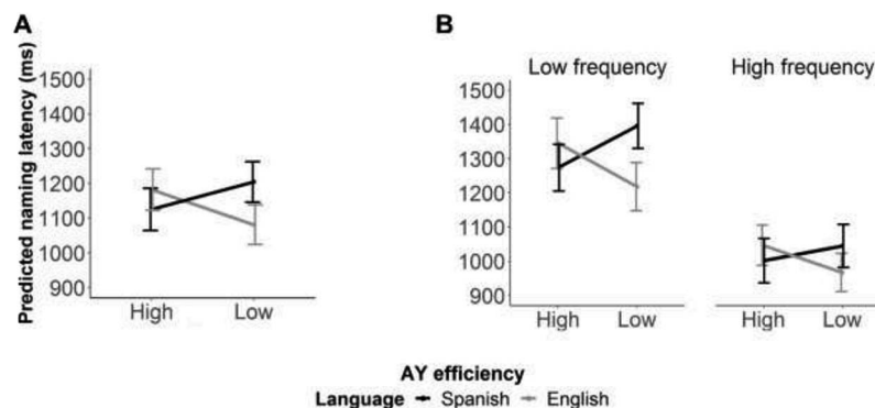
Figure 5. (A) Two-way interaction between language and AY efficiency and (B) three-way interaction between language, frequency, and AY efficiency for bilinguals in the varied context. Error bars represent standard error of the mean. A and B represent cues; X and Y represent probes.
