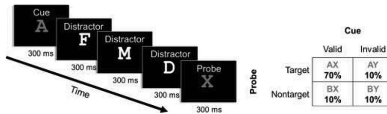
Figure 2. Schematic representation of the procedure for the AX variant of the continuous performance task. AX trials are target trials that require a “yes” probe response (70% of trials). All other trial sequences (each occurring 10% of the time) require a “no” probe response. AY trials share the cue with target trials, which biases participants to anticipate the target probe. High error rates in these trials indicate failure to suppress an incorrect “yes” response due to high reliance on context. In BX trials, the cue signals a “no” response, but the probe prompts a target response. High error rates in these trials indicate failure to suppress a “yes” response due to minimal or no reliance on context. BY trials are control trials where the influence of context is reduced, because both the cue and probe differ from target trials. A and B represent cues; X and Y represent probes; F, M, and D represent distractors.
