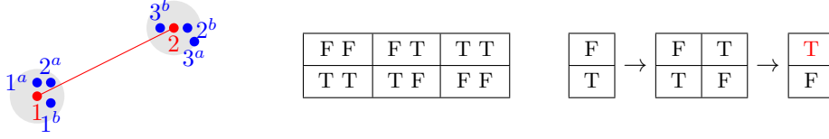
■ Figure 8 Left: An indecisive and a precise curve. Middle: Distance matrix. “T T” in the bottom left cell means \|1 - 1^a\| \leq \delta and \|1 - 1^b\| \leq \delta . Right: Computing reachability matrix, column by column. Note two reachability vectors for the second column.
