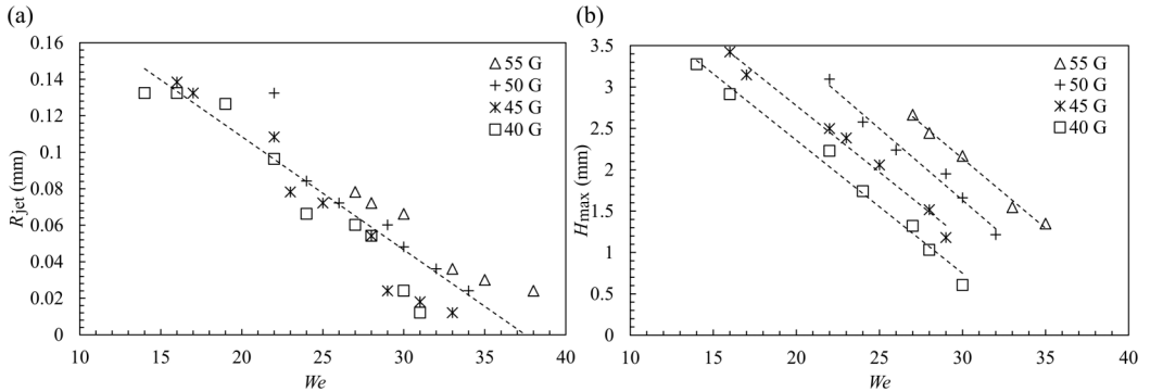
FIG. 9. (a) R_{\text{jet}} and (b) H_{\text{max}} against We , respectively. Linear fits added for discussion.
