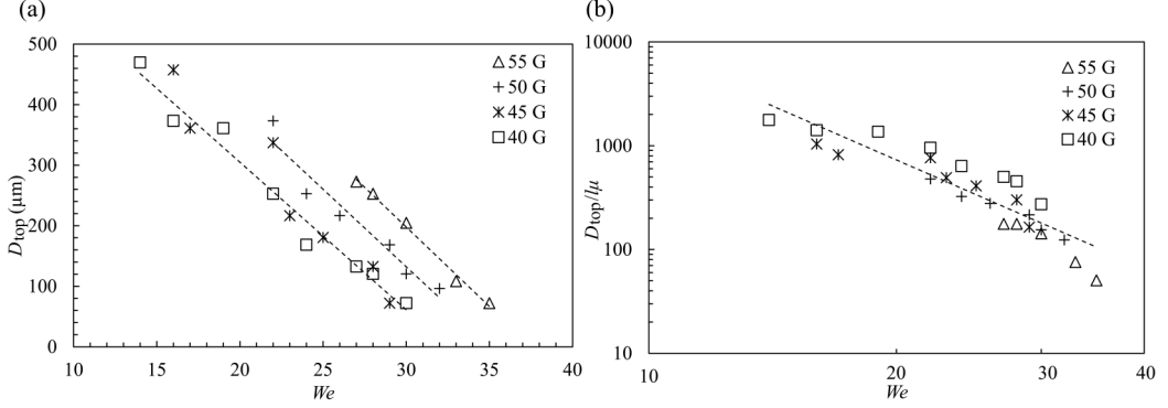
FIG. 12. (a) D_{\text{top}} versus We for test fluids. (b) Dimensionless D/l_{\mu} versus We with power fit D_{\text{top}}/l_{\mu} \approx We^{-3.45} .
