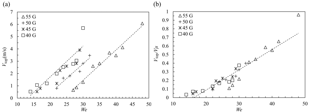
FIG. 13. (a) V_{\text{top}} versus We for test fluids. (b) Dimensionless velocity V_{\text{top}}/V_{\mu} versus We , with linear fit V_{\text{top}}/V_{\mu} \approx 0.023 We .
