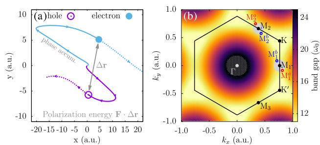
FIG. 1. (a) An imperfect recollision in which the electron and hole centers do not exactly overlap, leading to an electron-hole-pair polarization energy upon recollision. In the ERM, we also keep track of the phase accumulated along the trajectories. (b) Band gap energy (in units of \omega_0 = 0.0285 ) of monolayer hBN with annotated points of interest. The gray discs around M_1 and M_2 each has radius 0.1.
