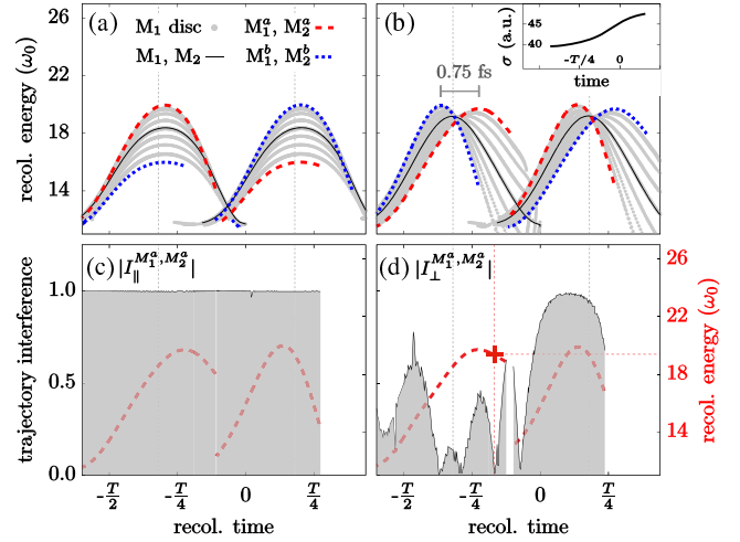
FIG. 3. Semiclassical recollision energies versus recollision times (a) without and (b) with inclusion of the EH-PER \mathbf{F} \cdot \Delta\mathbf{r} in Eq. (3c), for LPD along \Gamma - K direction. The different curves correspond to different tunneling sites in the BZ [Fig. 1(b)]. The vertical dotted lines mark the peaks of M_1 and M_2 recollision energies. The inset in (b) shows the spatial spread corresponding to the trajectory that tunnels at M_1 with the highest recollision energy (see text). The shaded curves in (c),(d) show the quantum interferences between the M_1^a and M_2^a emissions, for the (c) parallel and (d) perpendicular directions (see text). The recollision energies (right y axis) for M_1^a and M_2^a trajectories are redrawn in red dashed lines. (d) Red cross indicates the same interference minimum as in Fig. 2(d).
