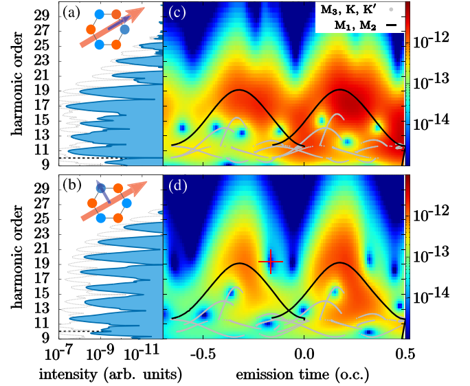
FIG. 2. HHG spectra (a),(b) and EPs (c),(d) for LPD along the \Gamma - K direction, and high harmonics polarized parallel (a),(c) and perpendicular (b),(d) to the LPD. (a),(b) Filled curve results from the full SBE calculation, the dotted line neglects the Berry connections, and the dashed horizontal line outlines the minimal band gap. (c),(d), Color map is the quantum result; the lines and dots are semiclassical results, with tunneling from different symmetry points in the BZ [see Fig. 1(b)]. (d) Red cross marks a minimum in the color map.
