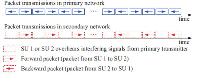
Fig. 3: A MAC protocol for spectrum sharing in a CRN that has two primary users and two secondary users.
