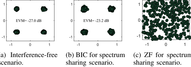
Fig. 13: Constellation diagram of the decoded signals at the secondary receiver (SU 2) in three different experiments.
