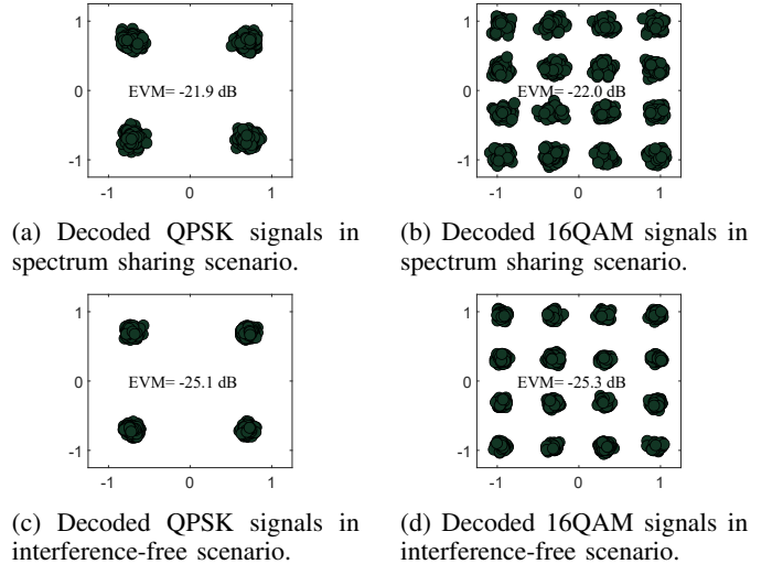
Fig. 16: Constellation diagram of decoded signals at SU 2: our spectrum sharing scheme versus interference-free scenario.
