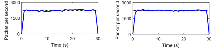
(a) Packet delivery rate in interference-free scenario. (b) Packet delivery rate in spectrum sharing scenario.
