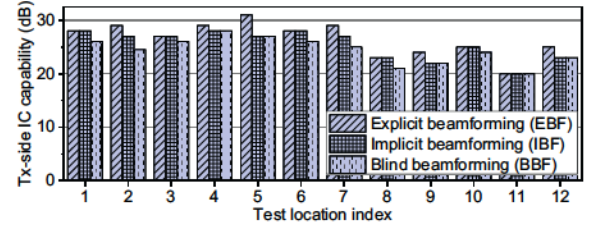
Fig. 19: Tx-side IC capability of the three beamforming techniques when the secondary device has three antennas.
