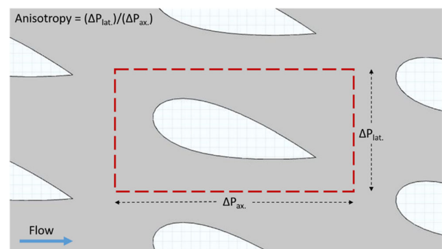
Fig. 2 Example of a repeating array unit used to determine values of anisotropy for different airfoil angles of attack, where \Delta P is the pressure drop across the array unit
