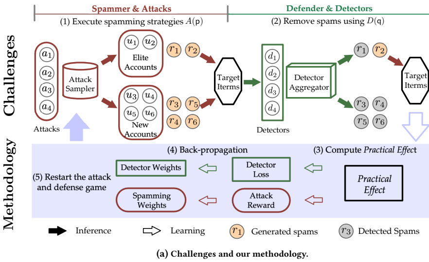
Figure 1: (a): A vulnerable spam detection pipeline, with steps numbered as (1), (2), etc. Accuracy-based detectors can be misled to detect numerous insignificant spams from new accounts, leaving behind the more manipulative elite spams. We define a zero-sum game to find a robust defender against unknown and evolving spamming strategies A(p) . (b): The Practical Effect vs. Recall of individual detectors (shown in legend) against a mixed spamming strategy. The curve is obtained by sweeping the detection thresholds. For most detectors, the attack could attain high practical effects even with high detection recall scores. (c): For a fixed spam detector (Fraudar), a spammer can choose the best out of five attack strategies to maximize the practical effect.
